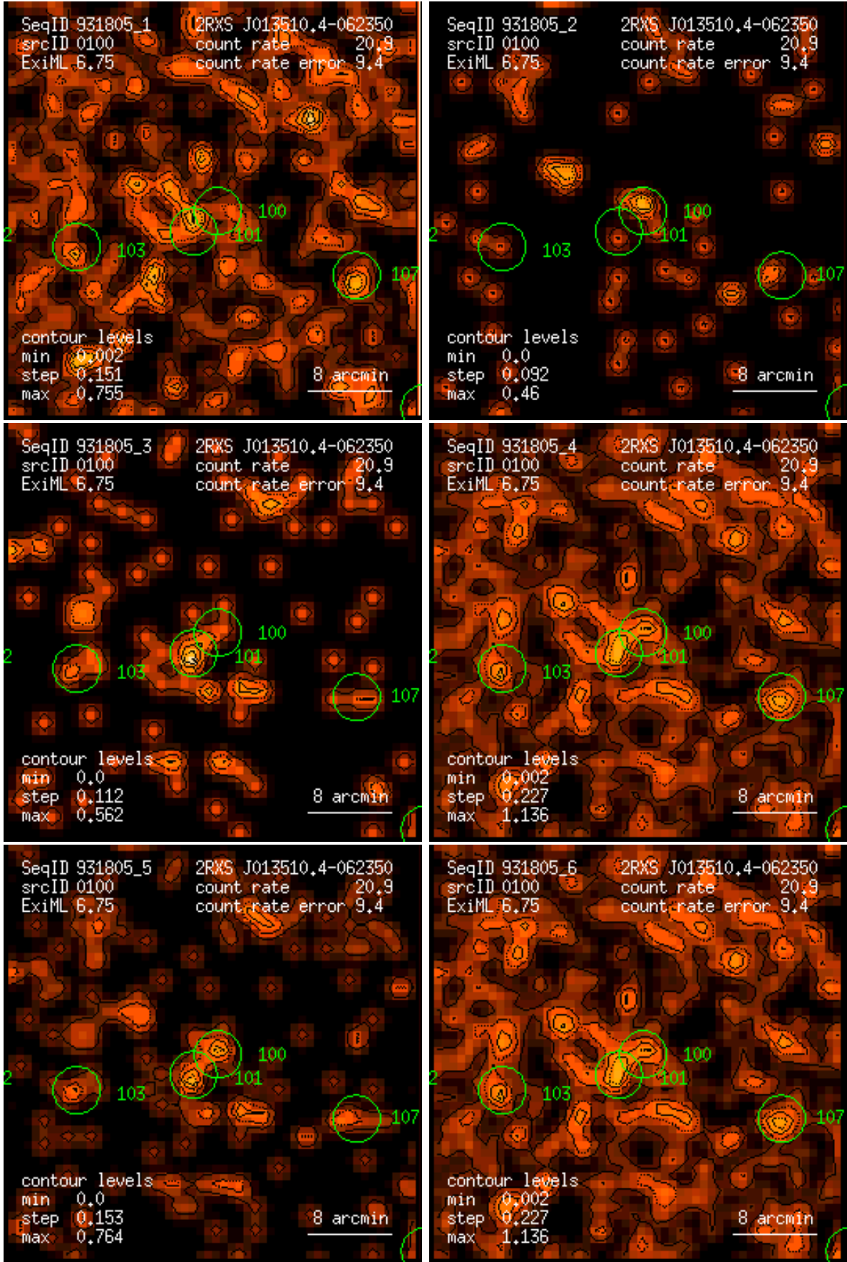
Figure 100: RASS 931805: detection 0100: band rate images, Gaussian filter: (1) PSPC channels 11 – 41, (2) 52 – 90, (3) 91 – 201, (4) 11 – 235, (5) 52 – 201, (6) 11 – 201. Broad band rates in counts/ks. Band rate contour levels in counts/ks/arcmin 2 .
