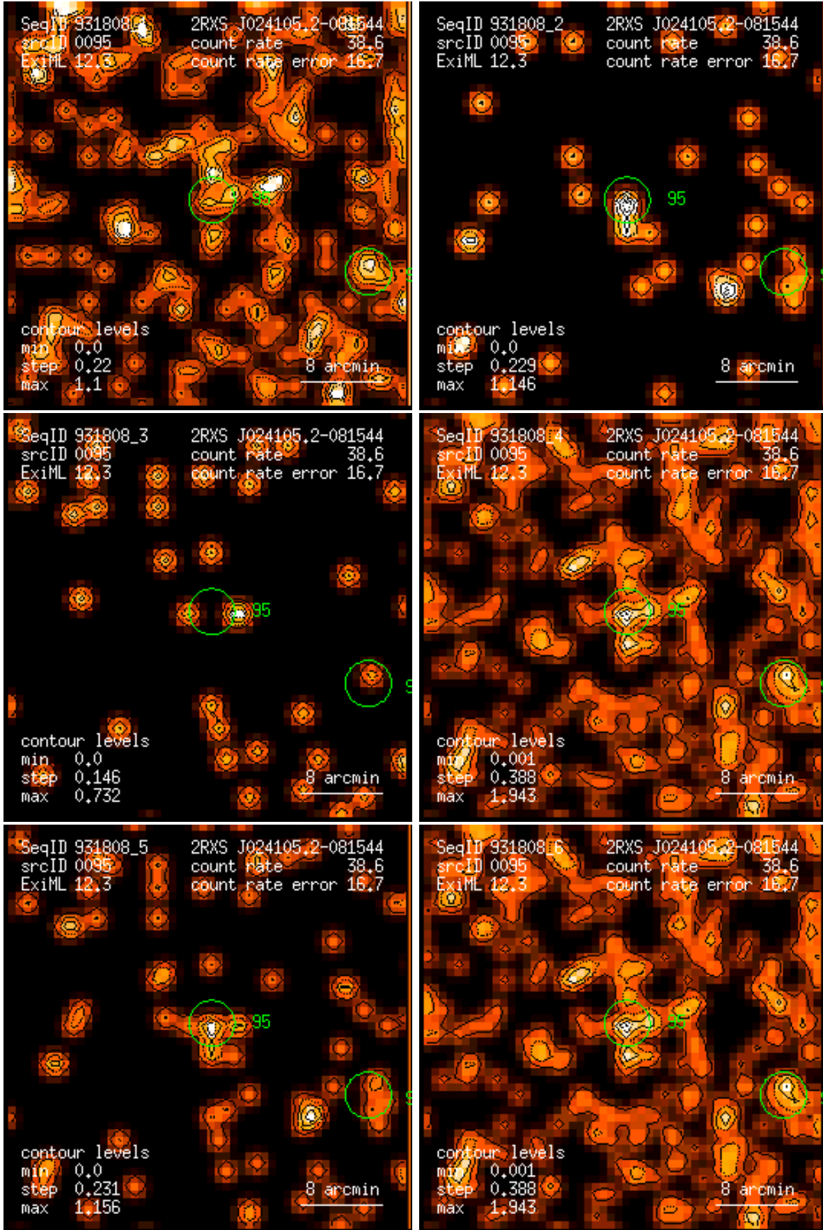
Figure 95: RASS 931808: detection 0095: band rate images, Gaussian filter: (1) PSPC channels 11 – 41, (2) 52 – 90, (3) 91 – 201, (4) 11 – 235, (5) 52 – 201, (6) 11 – 201. Broad band rates in counts/ks. Band rate contour levels in counts/ks/arcmin 2 .
