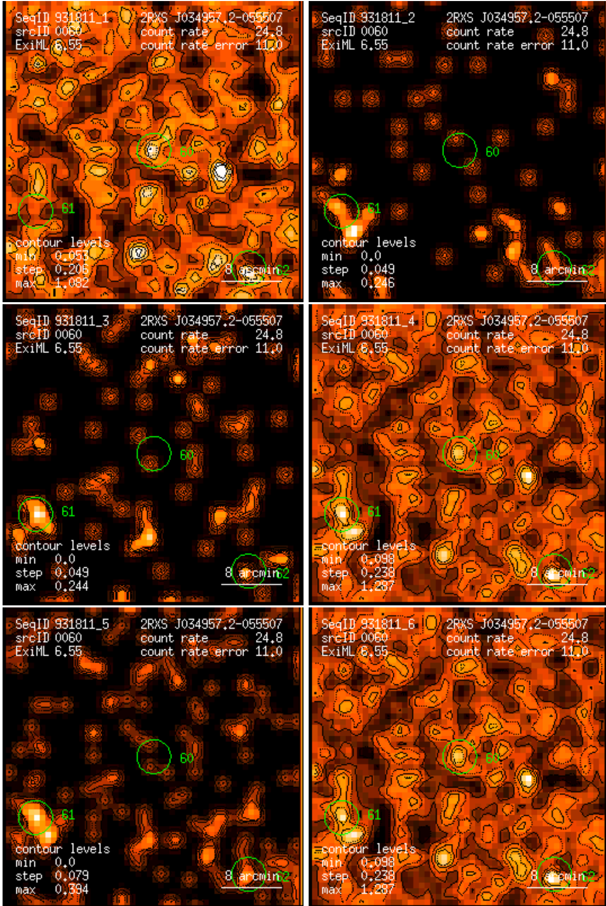
Figure 60: RASS 931811: detection 0060: band rate images, Gaussian filter: (1) PSC channels 11 – 41, (2) 52 – 90, (3) 91 – 201, (4) 11 – 235, (5) 52 – 201, (6) 11 – 201. Broad band rates in counts/ks. Band rate contour levels in counts/ks/arcmin 2 .
