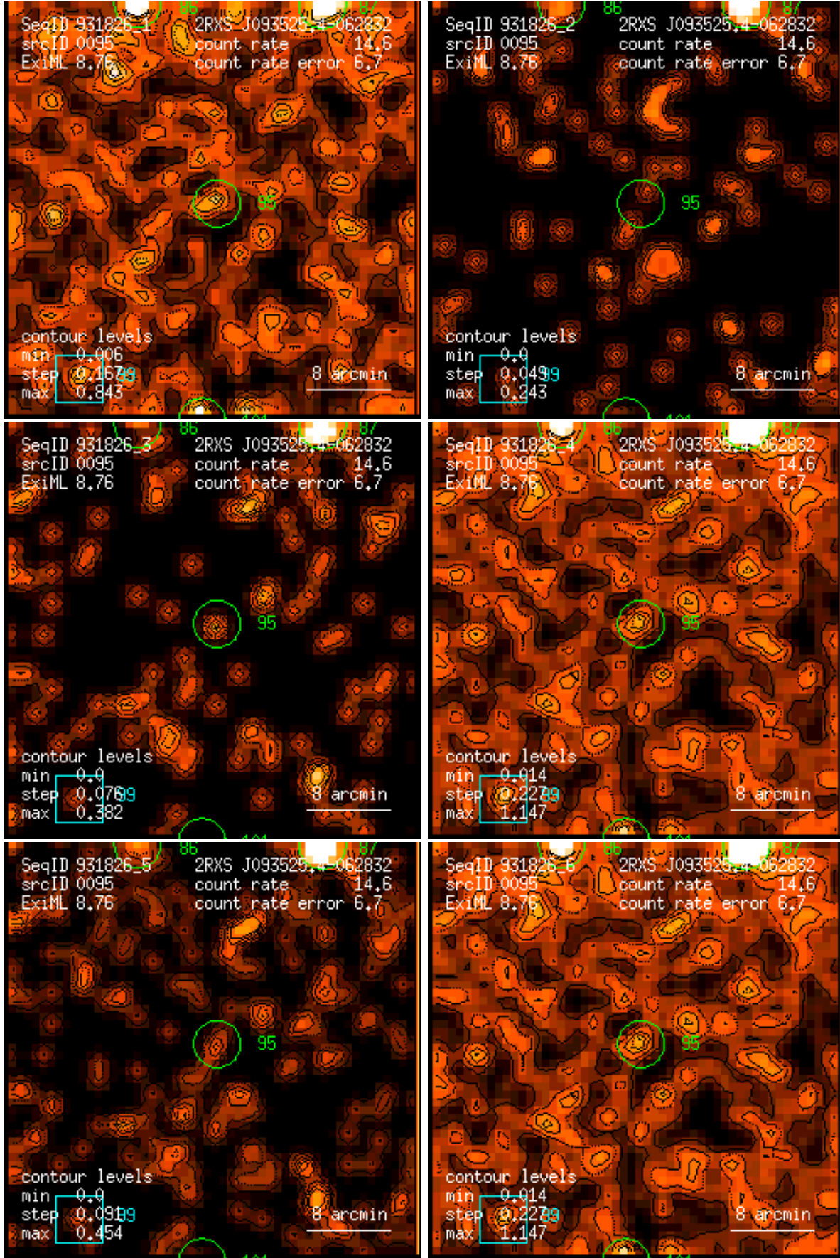
Figure 95: RASS 931826: detection 0095: band rate images, Gaussian filter: (1) PSPC channels 11 – 41, (2) 52 – 90, (3) 91 – 201, (4) 11 – 235, (5) 52 – 201, (6) 11 – 201. Broad band rates in counts/ks. Band rate contour levels in counts/ks/arcmin 2 .
