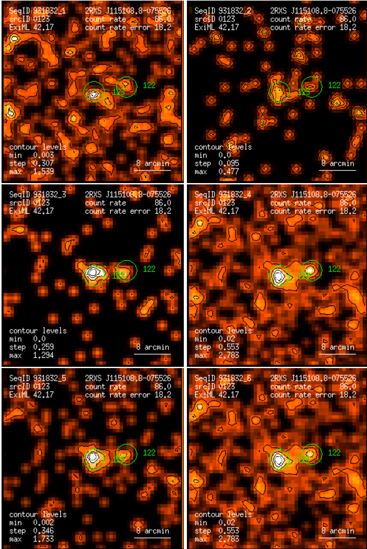
Figure 123: RASS 931832: detection 0123: band rate images, Gaussian filter: (1) PSPC channels 11 – 41, (2) 52 – 90, (3) 91 – 201, (4) 11 – 235, (5) 52 – 201, (6) 11 – 201. Broad band rates in counts/ks. Band rate contour levels in counts/ks/arcmin 2 .
