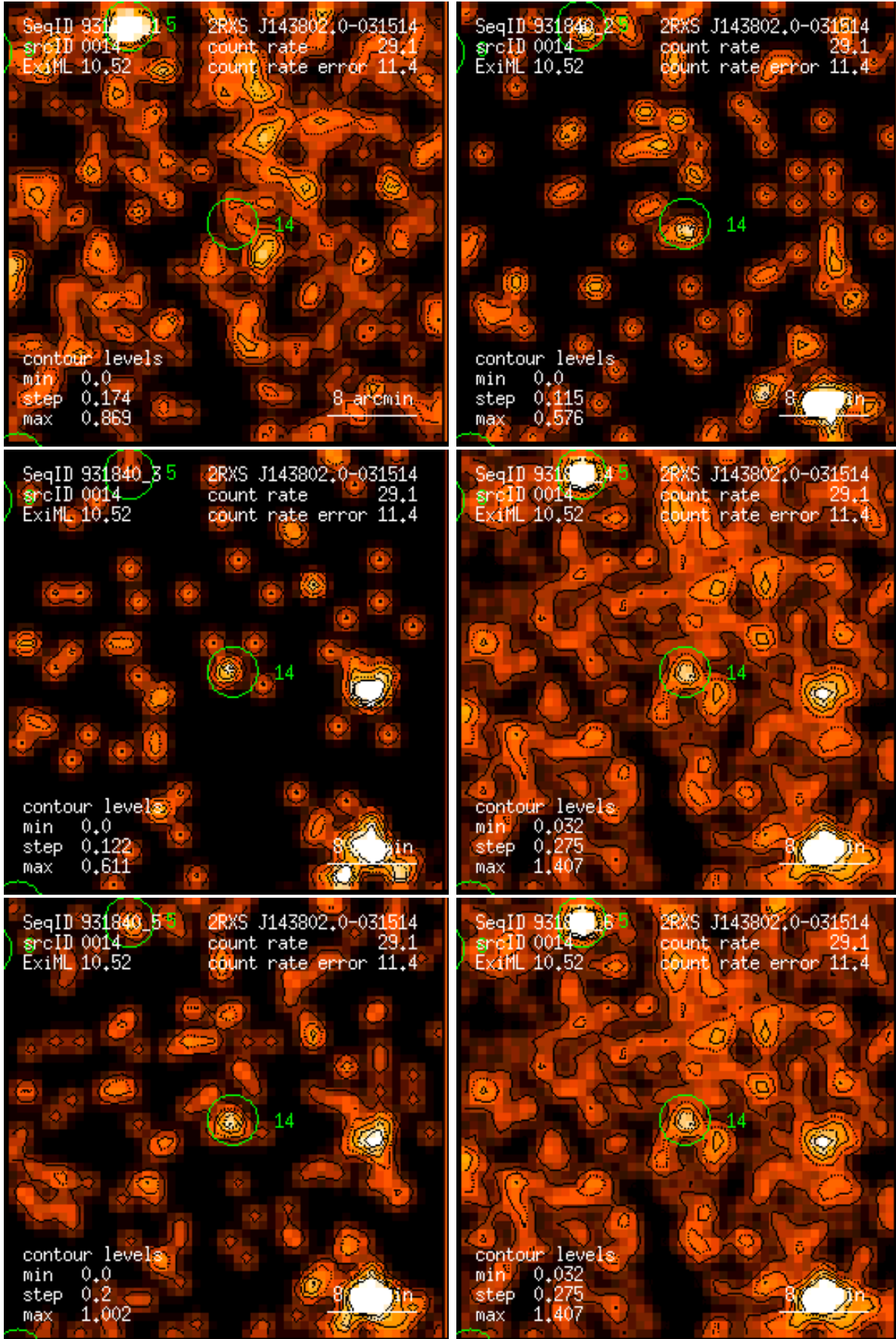
Figure 14: RASS 931840: detection 0014: band rate images, Gaussian filter: (1) PSPC channels 11 – 41, (2) 52 – 90, (3) 91 – 201, (4) 11 – 235, (5) 52 – 201, (6) 11 – 201. Broad band rates in counts/ks. Band rate contour levels in counts/ks/arcmin 2 .
