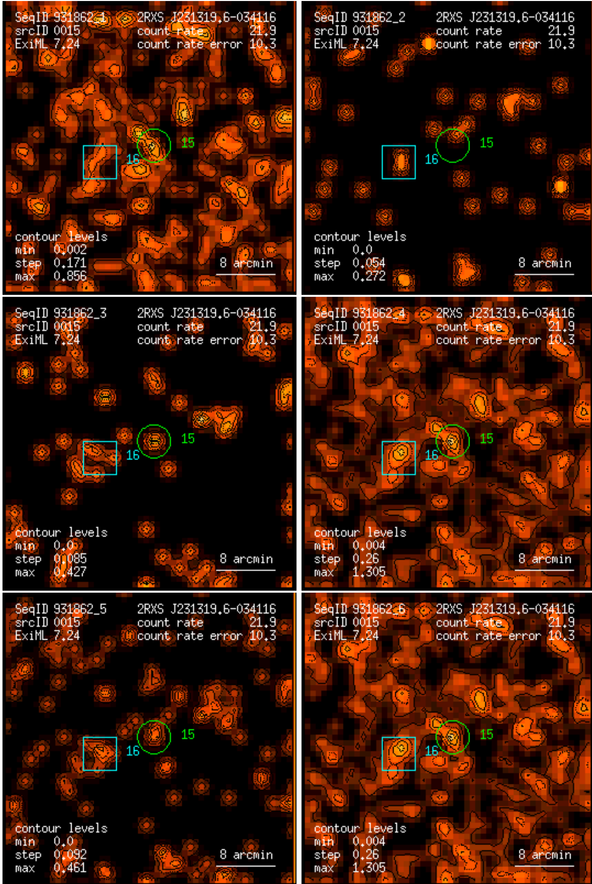
Figure 15: RASS 931862: detection 0015: band rate images, Gaussian filter: (1) PSPC channels 11 – 41, (2) 52 – 90, (3) 91 – 201, (4) 11 – 235, (5) 52 – 201, (6) 11 – 201. Broad band rates in counts/ks. Band rate contour levels in counts/ks/arcmin 2 .
