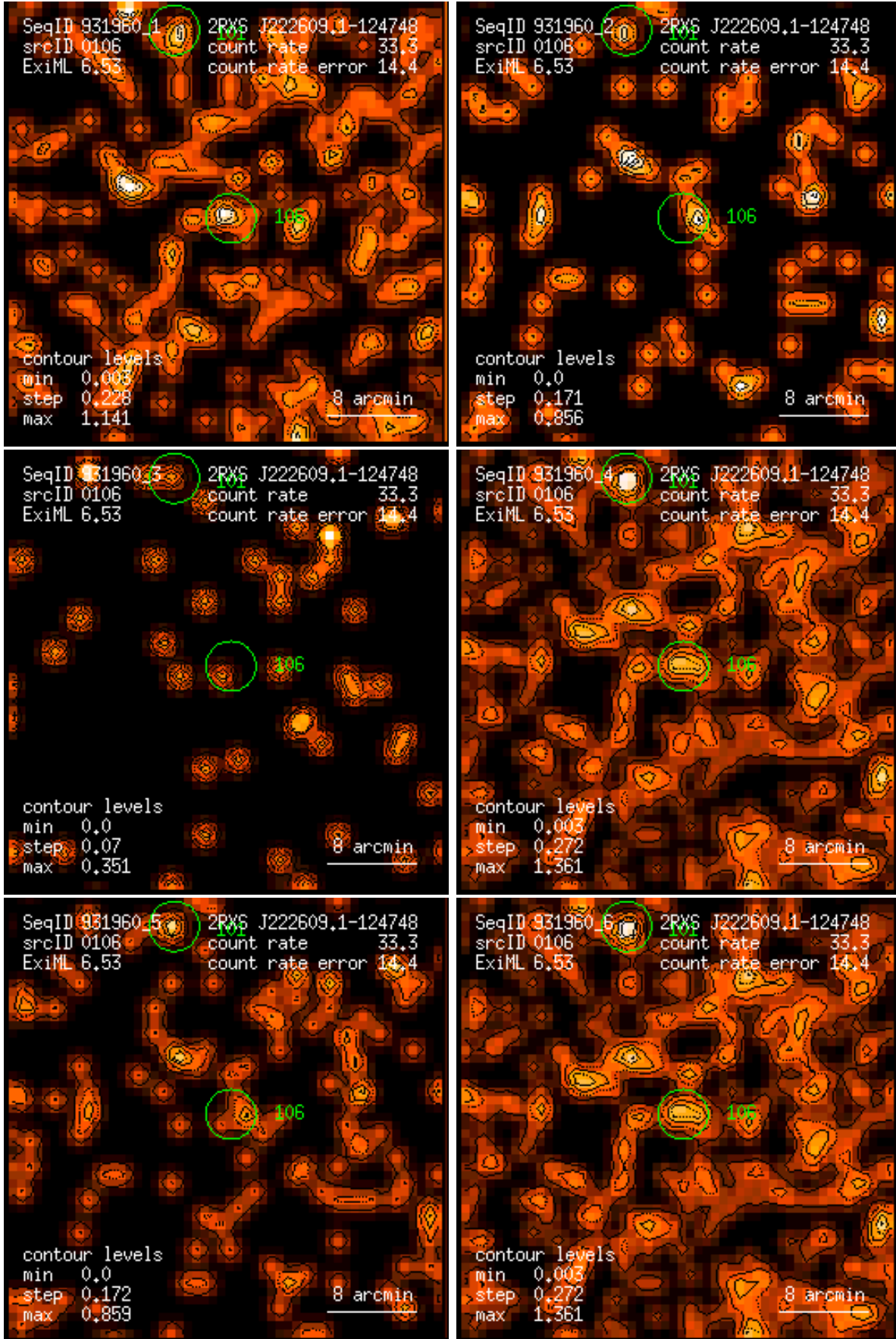
Figure 106: RASS 931960: detection 0106: band rate images, Gaussian filter: (1) PSPC channels 11 – 41, (2) 52 – 90, (3) 91 – 201, (4) 11 – 235, (5) 52 – 201, (6) 11 – 201. Broad band rates in counts/ks. Band rate contour levels in counts/ks/arcmin 2 .
