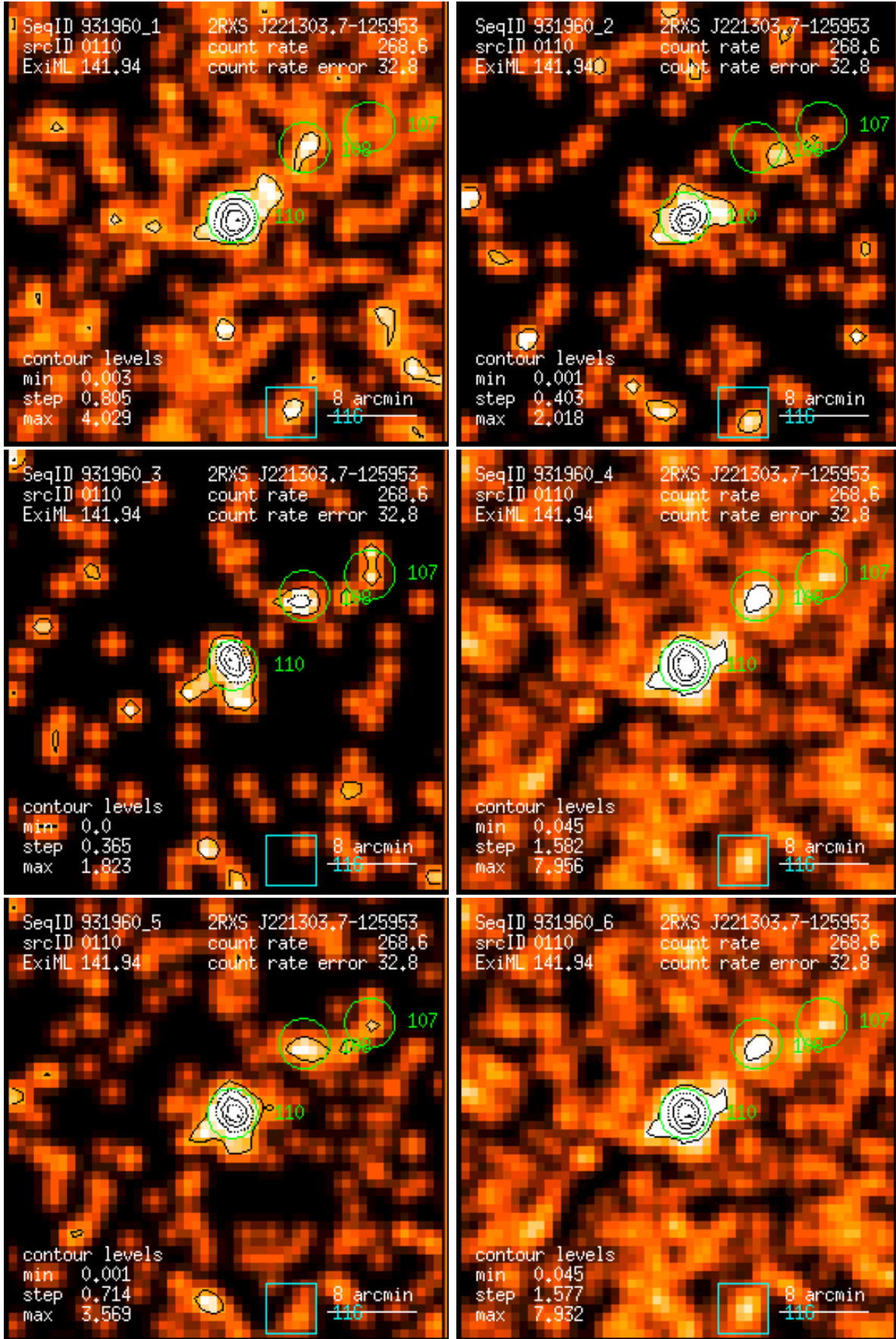
Figure 110: RASS 931960: detection 0110: band rate images, Gaussian filter: (1) PSPC channels 11 – 41, (2) 52 – 90, (3) 91 – 201, (4) 11 – 235, (5) 52 – 201, (6) 11 – 201. Broad band rates in counts/ks. Band rate contour levels in counts/ks/arcmin 2 .
