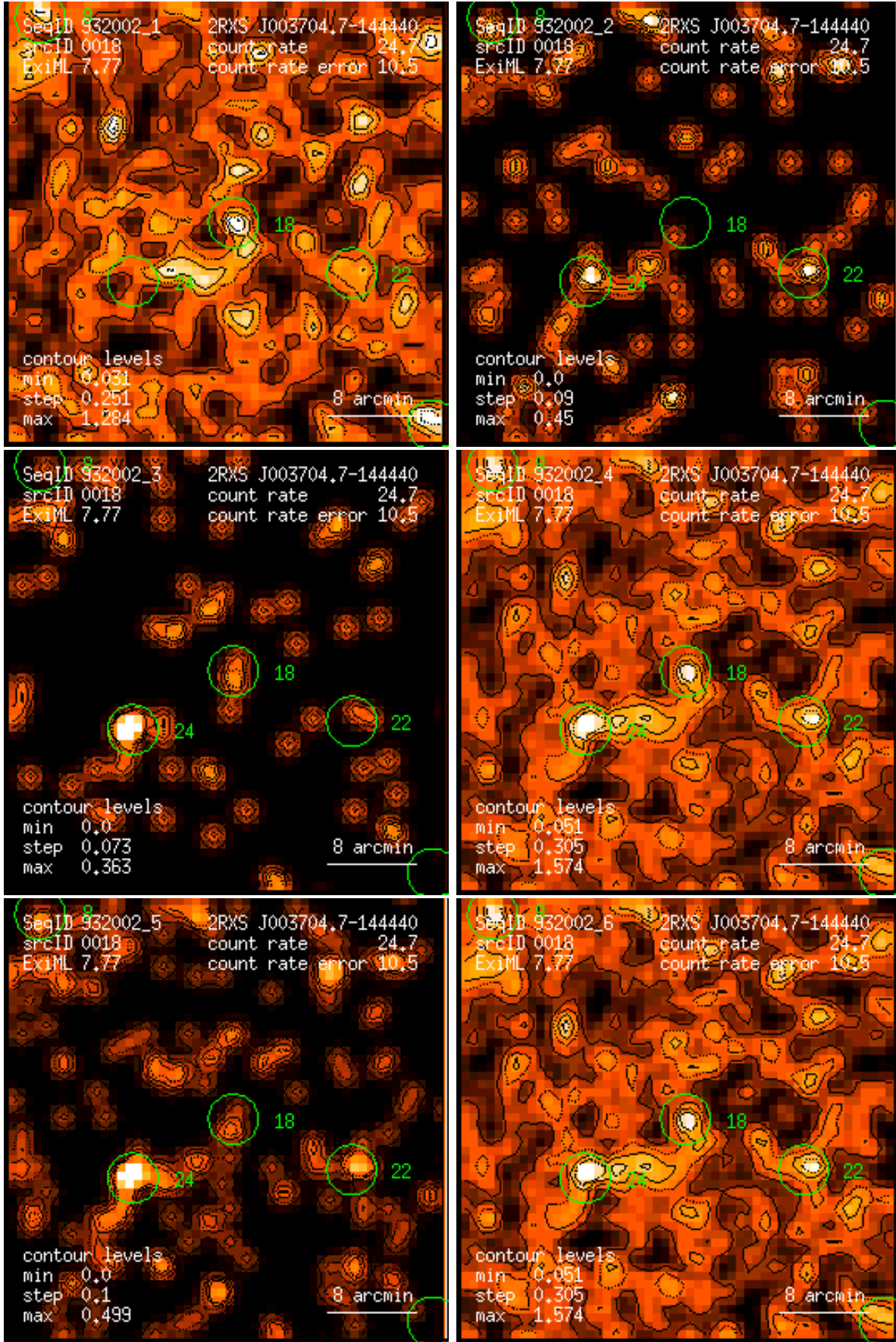
Figure 18: RASS 932002: detection 0018: band rate images, Gaussian filter: (1) PSPC channels 11 – 41, (2) 52 – 90, (3) 91 – 201, (4) 11 – 235, (5) 52 – 201, (6) 11 – 201. Broad band rates in counts/ks. Band rate contour levels in counts/ks/arcmin 2 .
