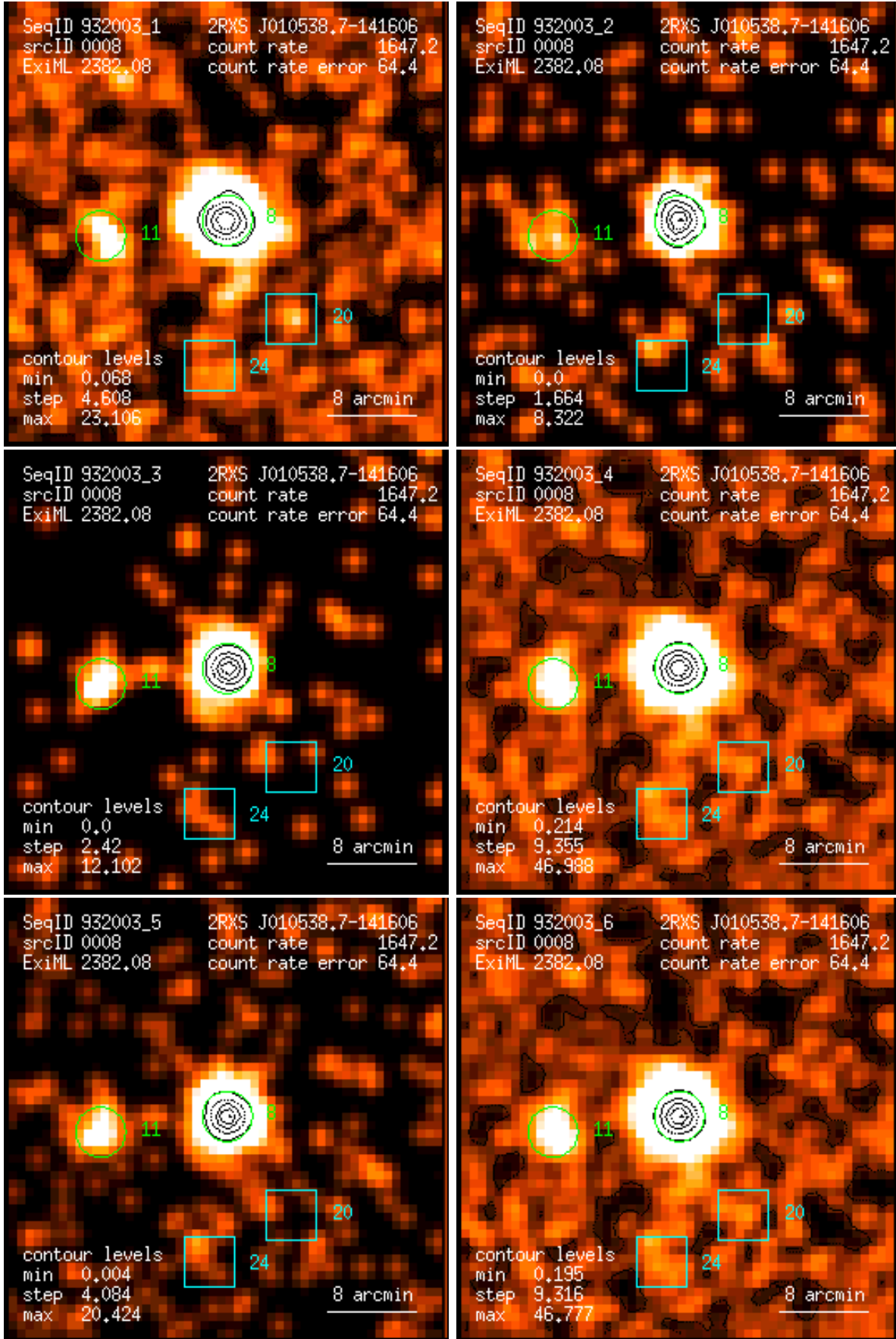
Figure 8: RASS 932003: detection 0008: band rate images, Gaussian filter: (1) PSPC channels 11 – 41, (2) 52 – 90, (3) 91 – 201, (4) 11 – 235, (5) 52 – 201, (6) 11 – 201. Broad band rates in counts/ks. Band rate contour levels in counts/ks/arcmin 2 .
