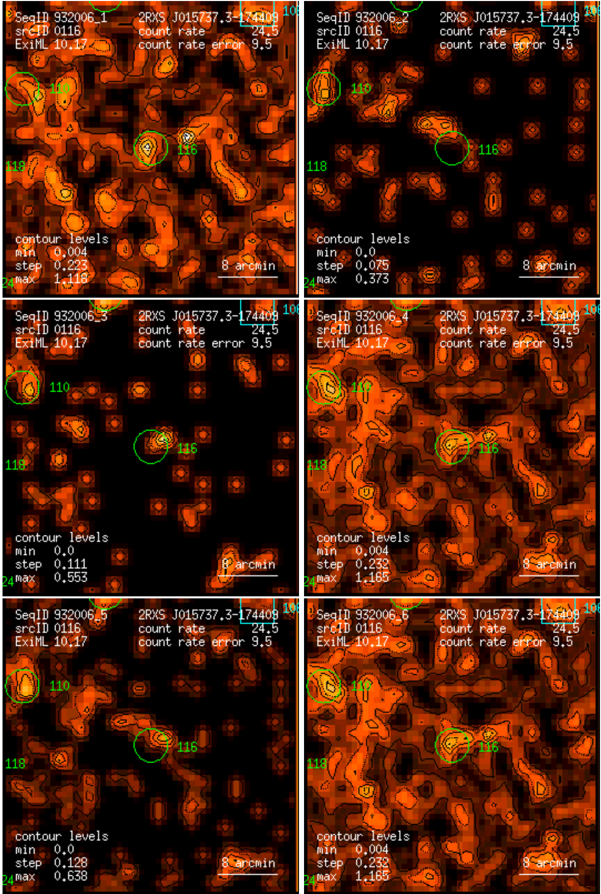
Figure 116: RASS 932006: detection 0116: band rate images, Gaussian filter: (1) PSPC channels 11 – 41, (2) 52 – 90, (3) 91 – 201, (4) 11 – 235, (5) 52 – 201, (6) 11 – 201. Broad band rates in counts/ks. Band rate contour levels in counts/ks/arcmin 2 .
