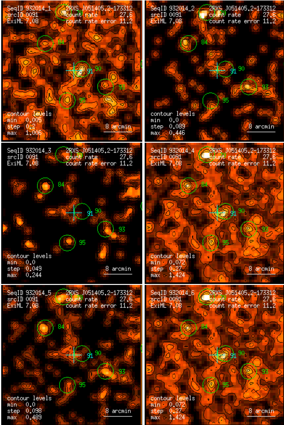
Figure 91: RASS 932014: detection 0091: band rate images, Gaussian filter: (1) PSCC channels 11 – 41, (2) 52 – 90, (3) 91 – 201, (4) 11 – 235, (5) 52 – 201, (6) 11 – 201. Broad band rates in counts/ks. Band rate contour levels in counts/ks/arcmin 2 .
