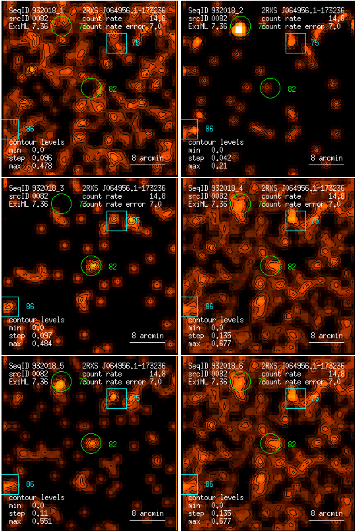
Figure 82: RASS 932018: detection 0082: band rate images, Gaussian filter: (1) PSPC channels 11 – 41, (2) 52 – 90, (3) 91 – 201, (4) 11 – 235, (5) 52 – 201, (6) 11 – 201. Broad band rates in counts/ks. Band rate contour levels in counts/ks/arcmin 2 .
