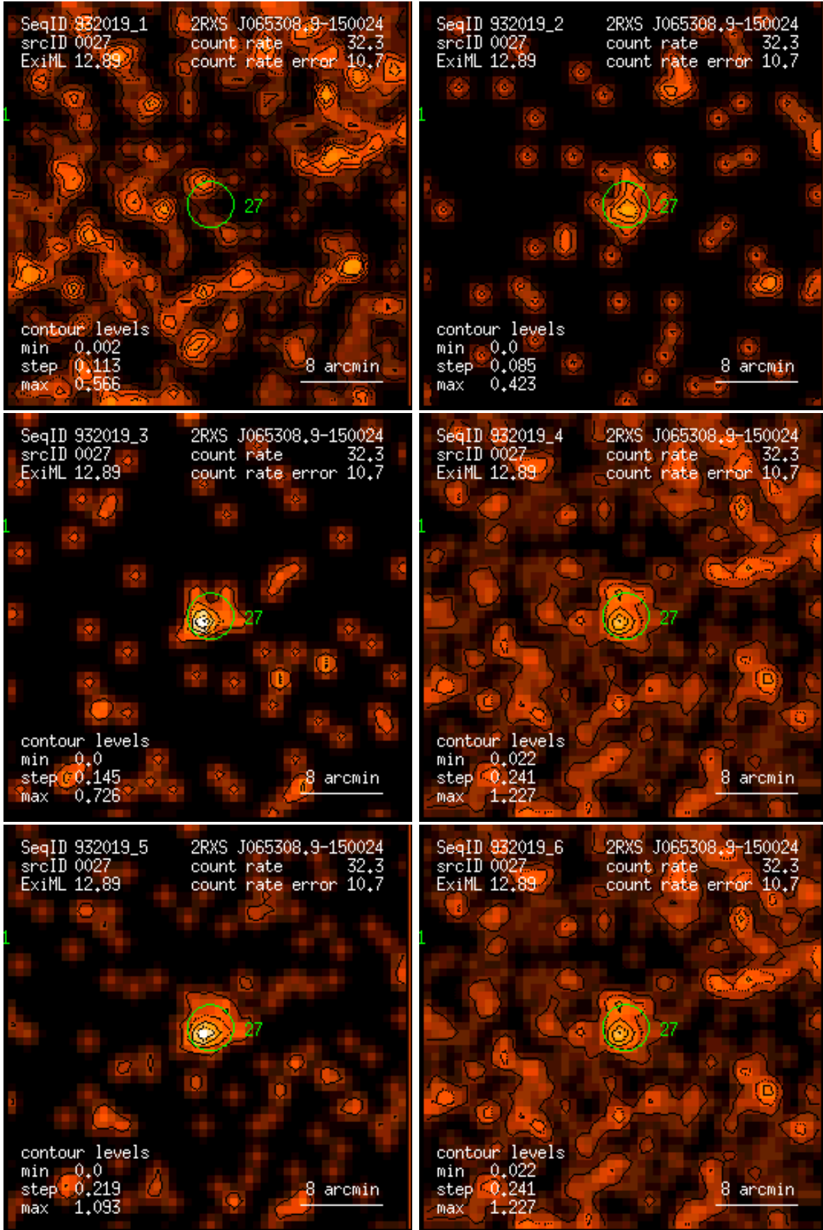
Figure 27: RASS 932019: detection 0027: band rate images, Gaussian filter: (1) PSPC channels 11 – 41, (2) 52 – 90, (3) 91 – 201, (4) 11 – 235, (5) 52 – 201, (6) 11 – 201. Broad band rates in counts/ks. Band rate contour levels in counts/ks/arcmin 2 .
