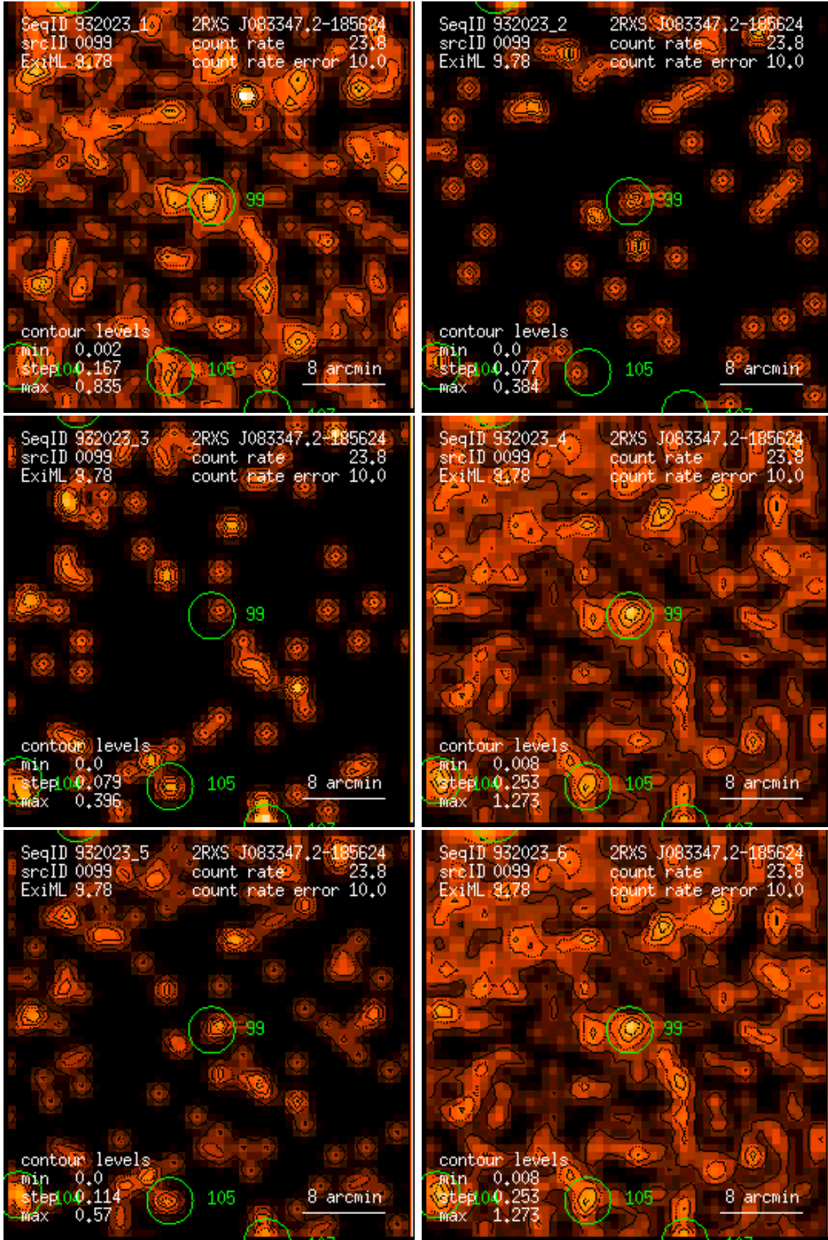
Figure 99: RASS 932023: detection 0099: band rate images, Gaussian filter: (1) PSPC channels 11 – 41, (2) 52 – 90, (3) 91 – 201, (4) 11 – 235, (5) 52 – 201, (6) 11 – 201. Broad band rates in counts/ks. Band rate contour levels in counts/ks/arcmin 2 .
