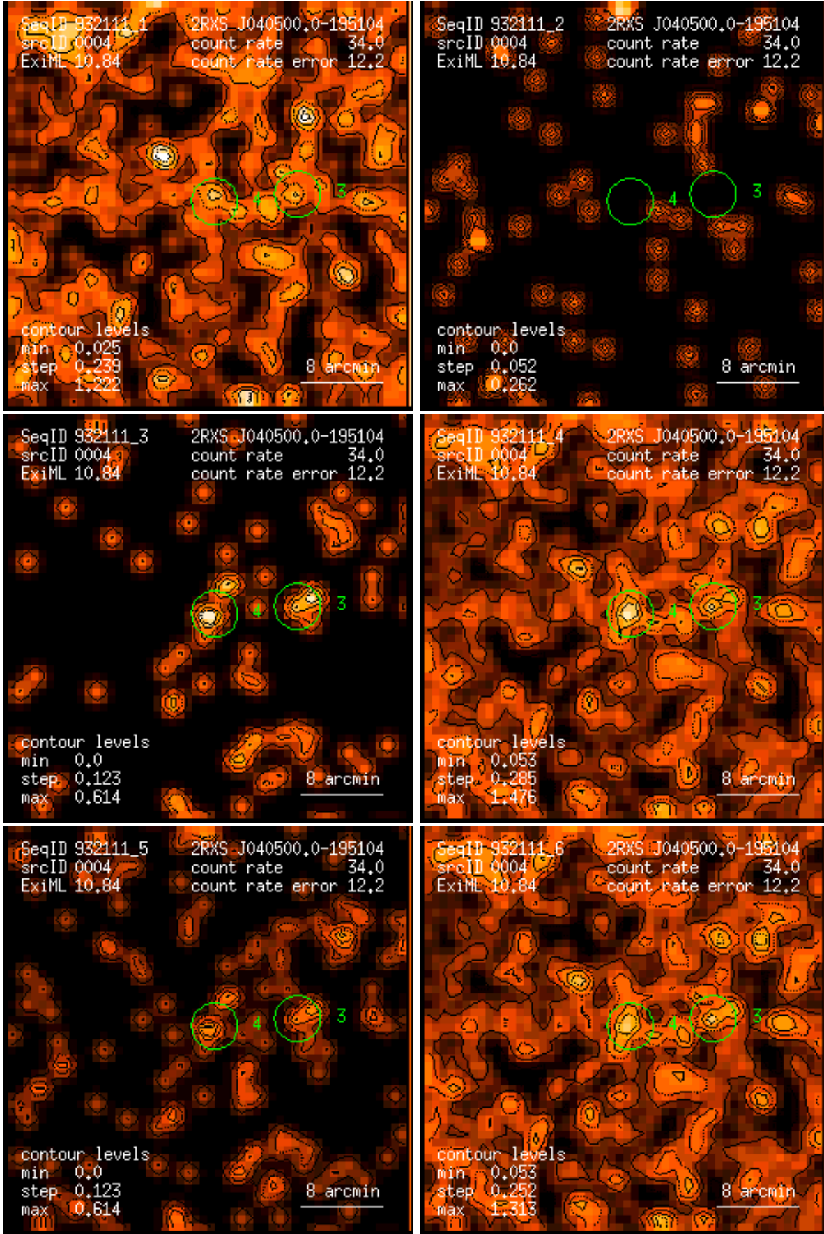
Figure 4: RASS 932111: detection 0004: band rate images, Gaussian filter: (1) PSPC channels 11 – 41, (2) 52 – 90, (3) 91 – 201, (4) 11 – 235, (5) 52 – 201, (6) 11 – 201. Broad band rates in counts/ks. Band rate contour levels in counts/ks/arcmin 2 .
