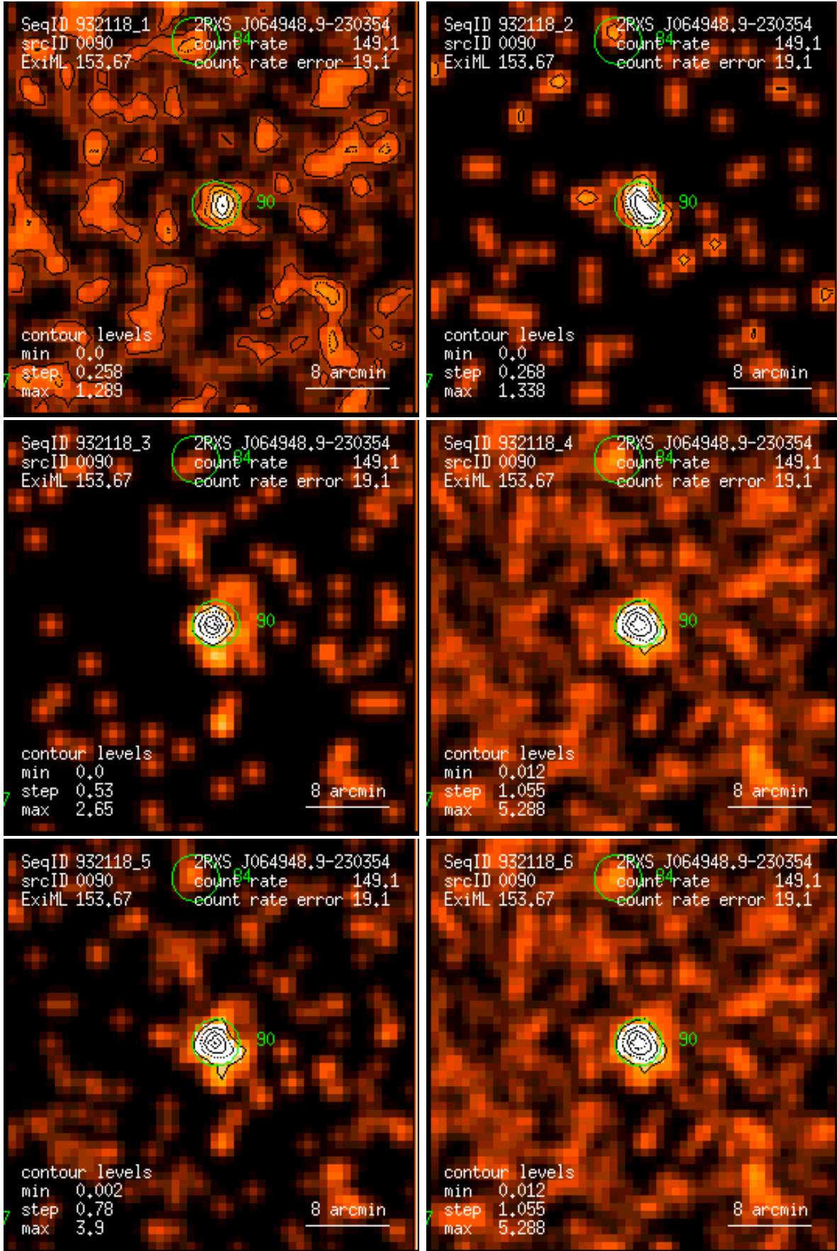
Figure 90: RASS 932118: detection 0090: band rate images, Gaussian filter: (1) PSPC channels 11 – 41, (2) 52 – 90, (3) 91 – 201, (4) 11 – 235, (5) 52 – 201, (6) 11 – 201. Broad band rates in counts/ks. Band rate contour levels in counts/ks/arcmin 2 .
