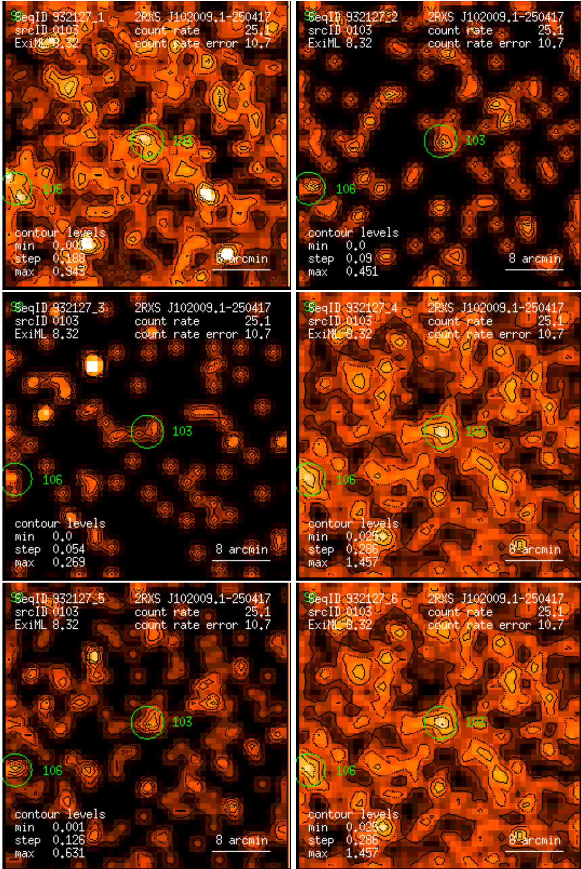
Figure 103: RASS 932127: detection 0103: band rate images, Gaussian filter: (1) PSPC channels 11 – 41, (2) 52 – 90, (3) 91 – 201, (4) 11 – 235, (5) 52 – 201, (6) 11 – 201. Broad band rates in counts/ks. Band rate contour levels in counts/ks/arcmin 2 .
