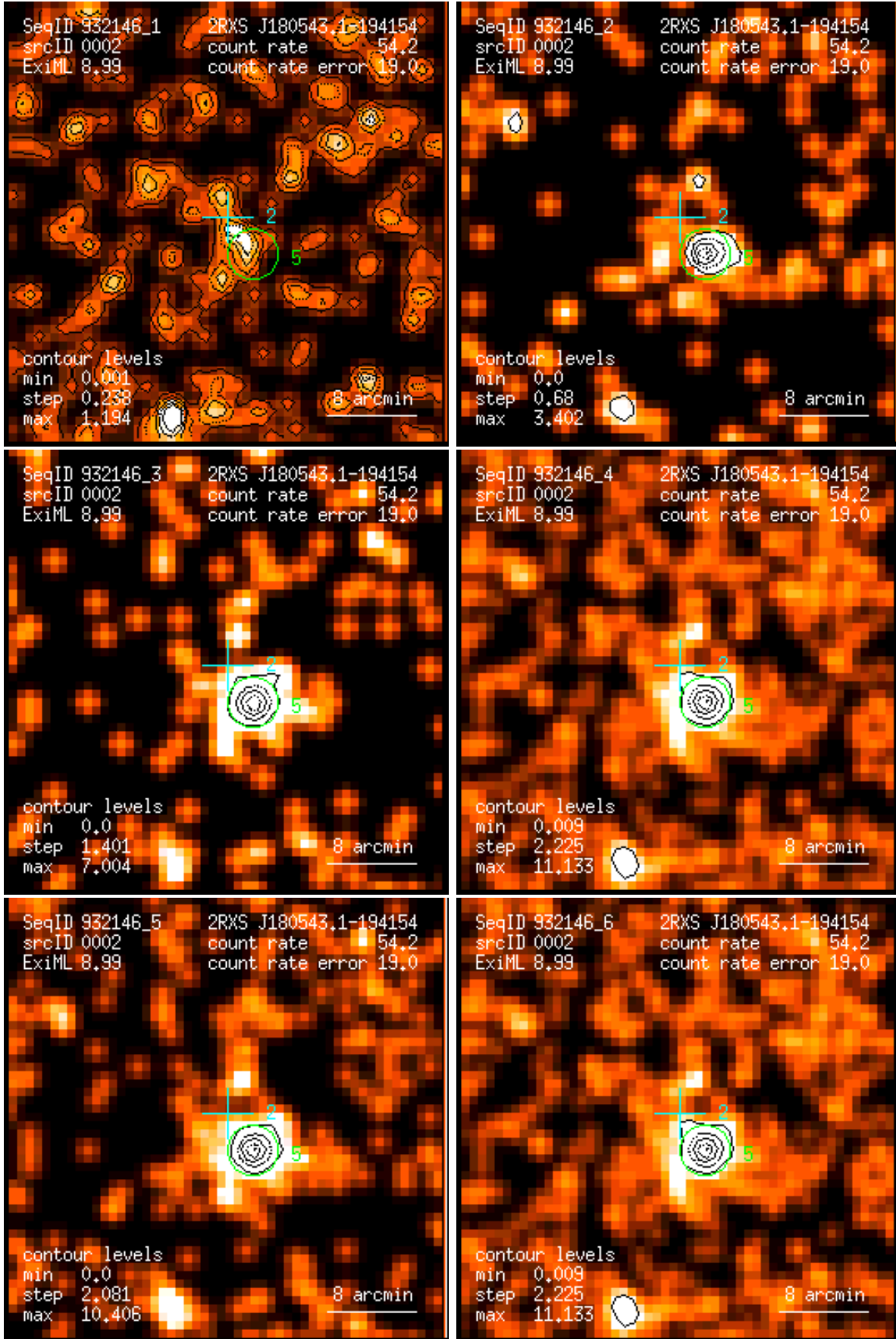
Figure 2: RASS 932146: detection 0002: band rate images, Gaussian filter: (1) PSPC channels 11 – 41, (2) 52 – 90, (3) 91 – 201, (4) 11 – 235, (5) 52 – 201, (6) 11 – 201. Broad band rates in counts/ks. Band rate contour levels in counts/ks/arcmin 2 .
