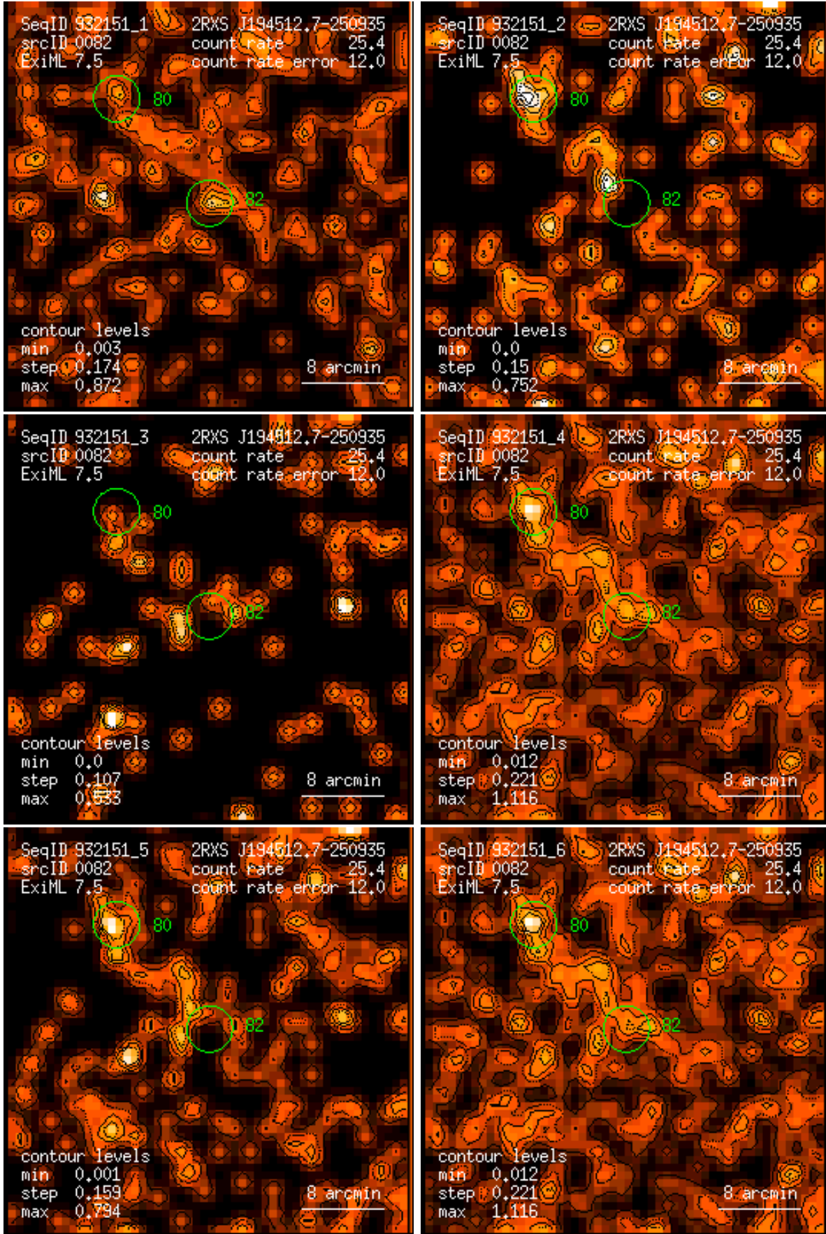
Figure 82: RASS 932151: detection 0082: band rate images, Gaussian filter: (1) PSPC channels 11 – 41, (2) 52 – 90, (3) 91 – 201, (4) 11 – 235, (5) 52 – 201, (6) 11 – 201. Broad band rates in counts/ks. Band rate contour levels in counts/ks/arcmin 2 .
