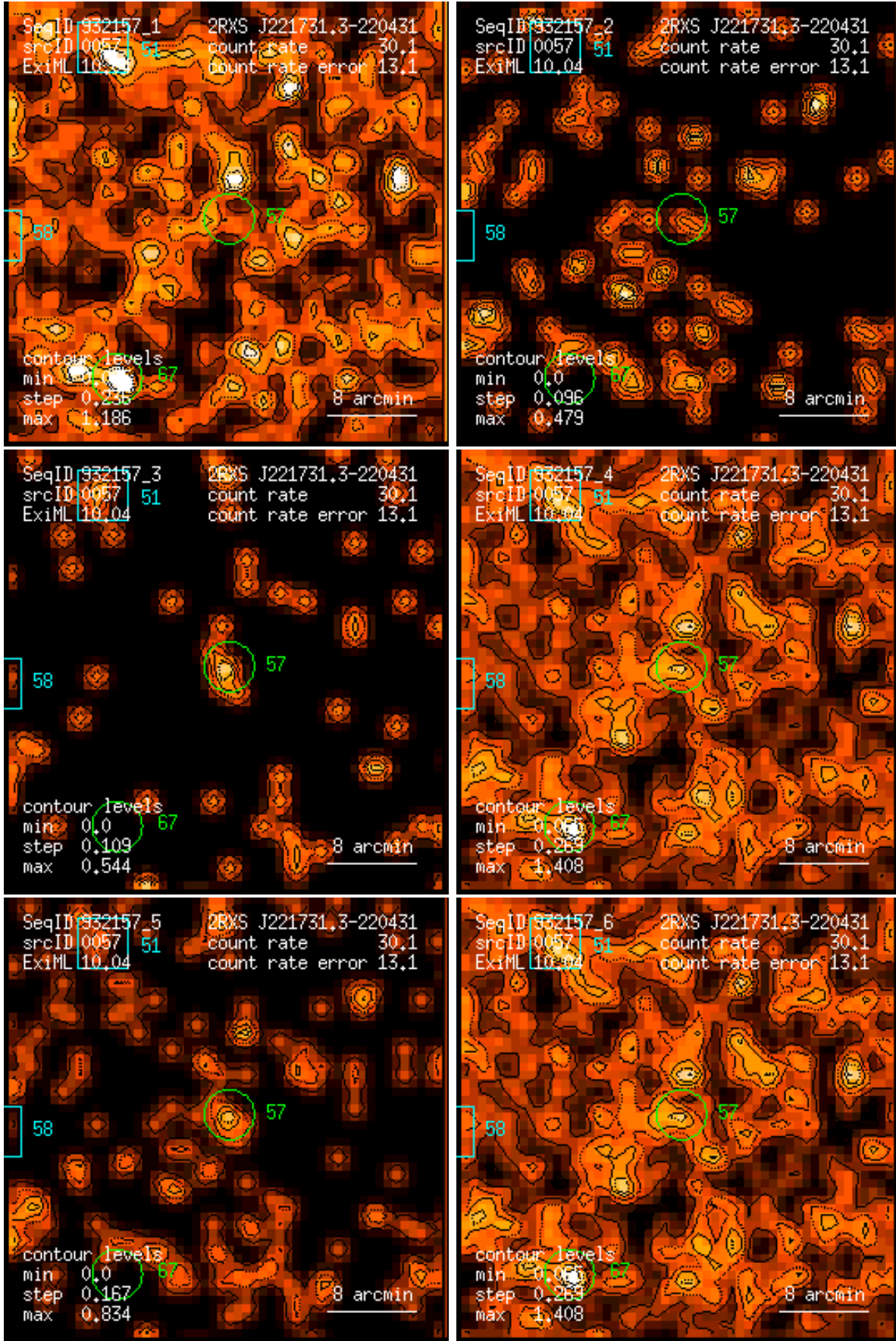
Figure 57: RASS 932157: detection 0057: band rate images, Gaussian filter: (1) PSPC channels 11 – 41, (2) 52 – 90, (3) 91 – 201, (4) 11 – 235, (5) 52 – 201, (6) 11 – 201. Broad band rates in counts/ks. Band rate contour levels in counts/ks/arcmin 2 .
