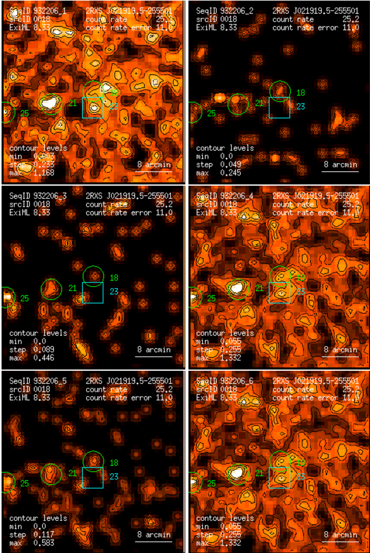
Figure 18: RASS 932206: detection 0018: band rate images, Gaussian filter: (1) PSPC channels 11 – 41, (2) 52 – 90, (3) 91 – 201, (4) 11 – 235, (5) 52 – 201, (6) 11 – 201. Broad band rates in counts/ks. Band rate contour levels in counts/ks/arcmin 2 .
