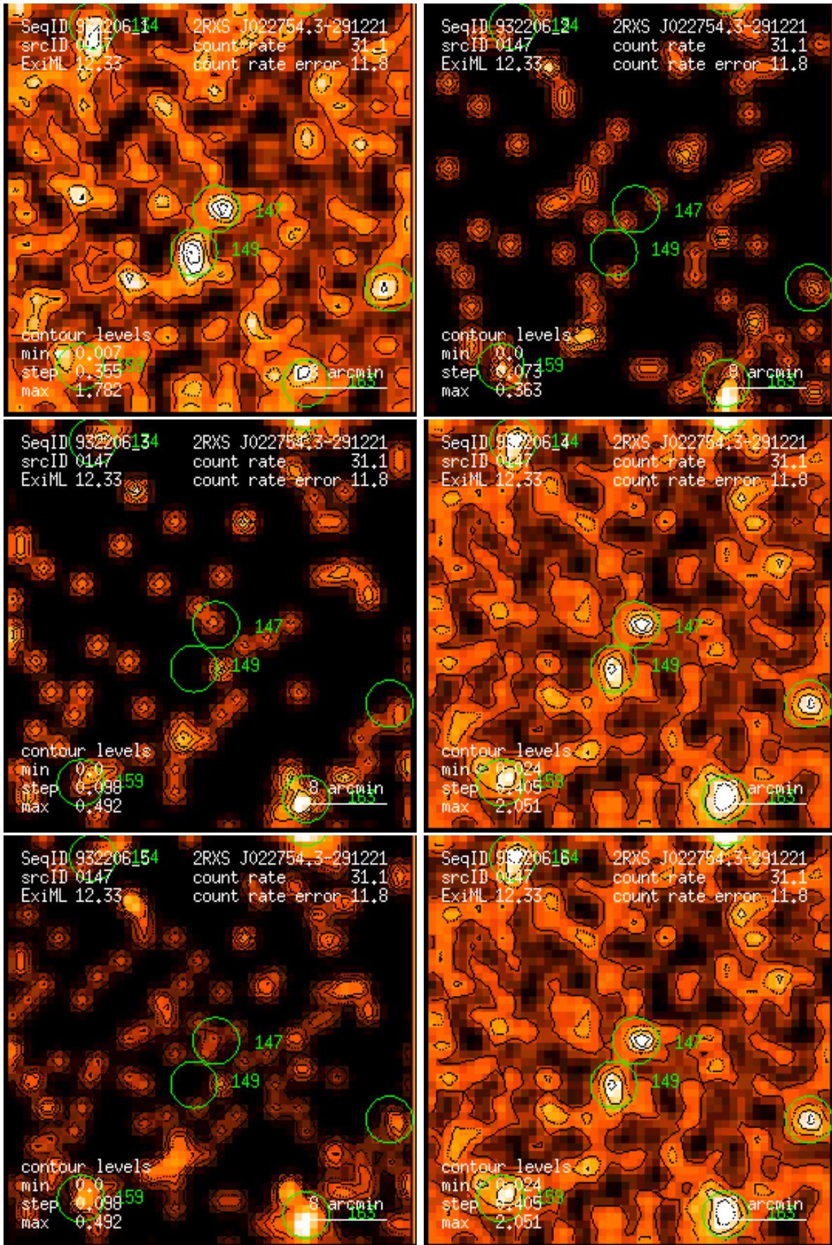
Figure 147: RASS 932206: detection 0147: band rate images, Gaussian filter: (1) PSPC channels 11 – 41, (2) 52 – 90, (3) 91 – 201, (4) 11 – 235, (5) 52 – 201, (6) 11 – 201. Broad band rates in counts/ks. Band rate contour levels in counts/ks/arcmin 2 .
