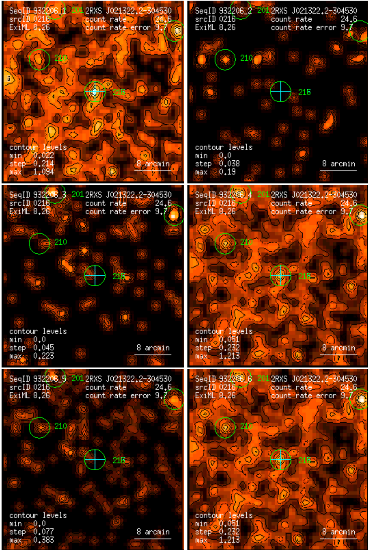
Figure 216: RASS 932206: detection 0216: band rate images, Gaussian filter: (1) PSPC channels 11 – 41, (2) 52 – 90, (3) 91 – 201, (4) 11 – 235, (5) 52 – 201, (6) 11 – 201. Broad band rates in counts/ks. Band rate contour levels in counts/ks/arcmin 2 .
