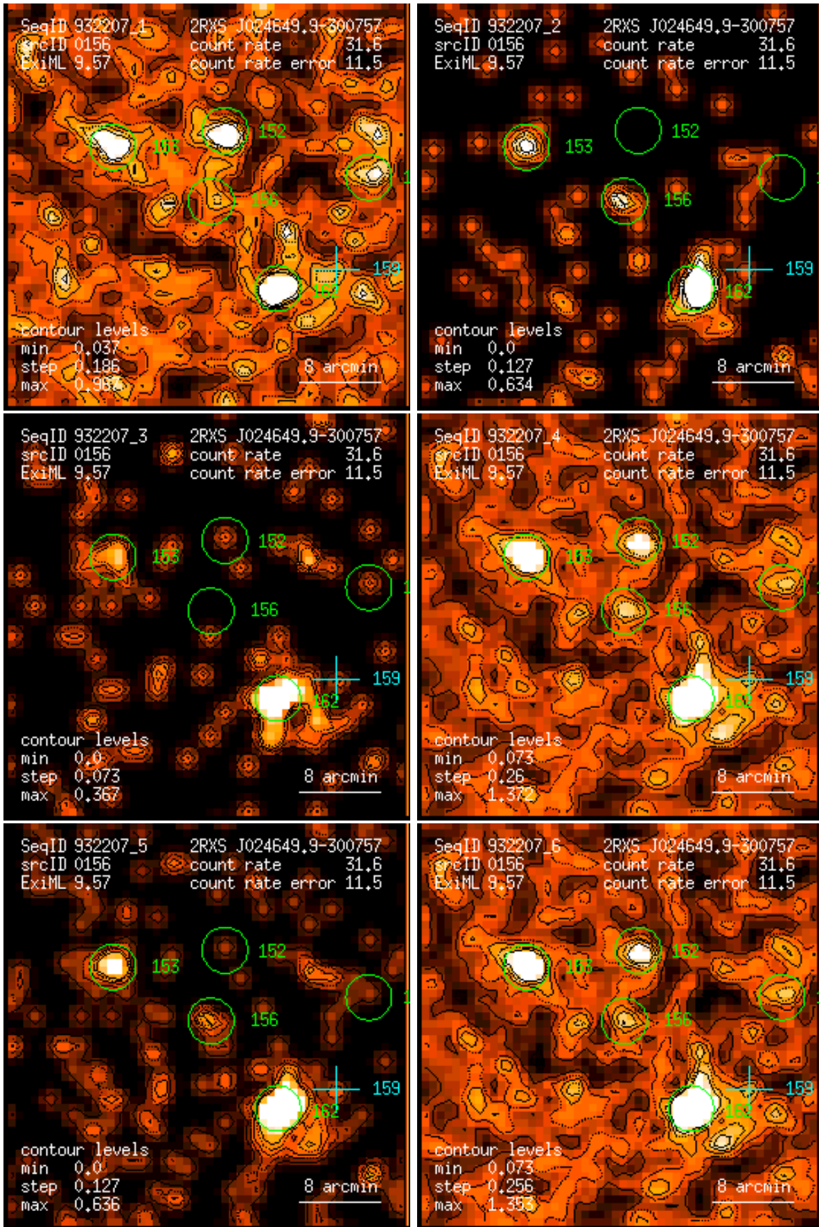
Figure 156: RASS 932207: detection 0156: band rate images, Gaussian filter: (1) PSPC channels 11 – 41, (2) 52 – 90, (3) 91 – 201, (4) 11 – 235, (5) 52 – 201, (6) 11 – 201. Broad band rates in counts/ks. Band rate contour levels in counts/ks/arcmin 2 .
