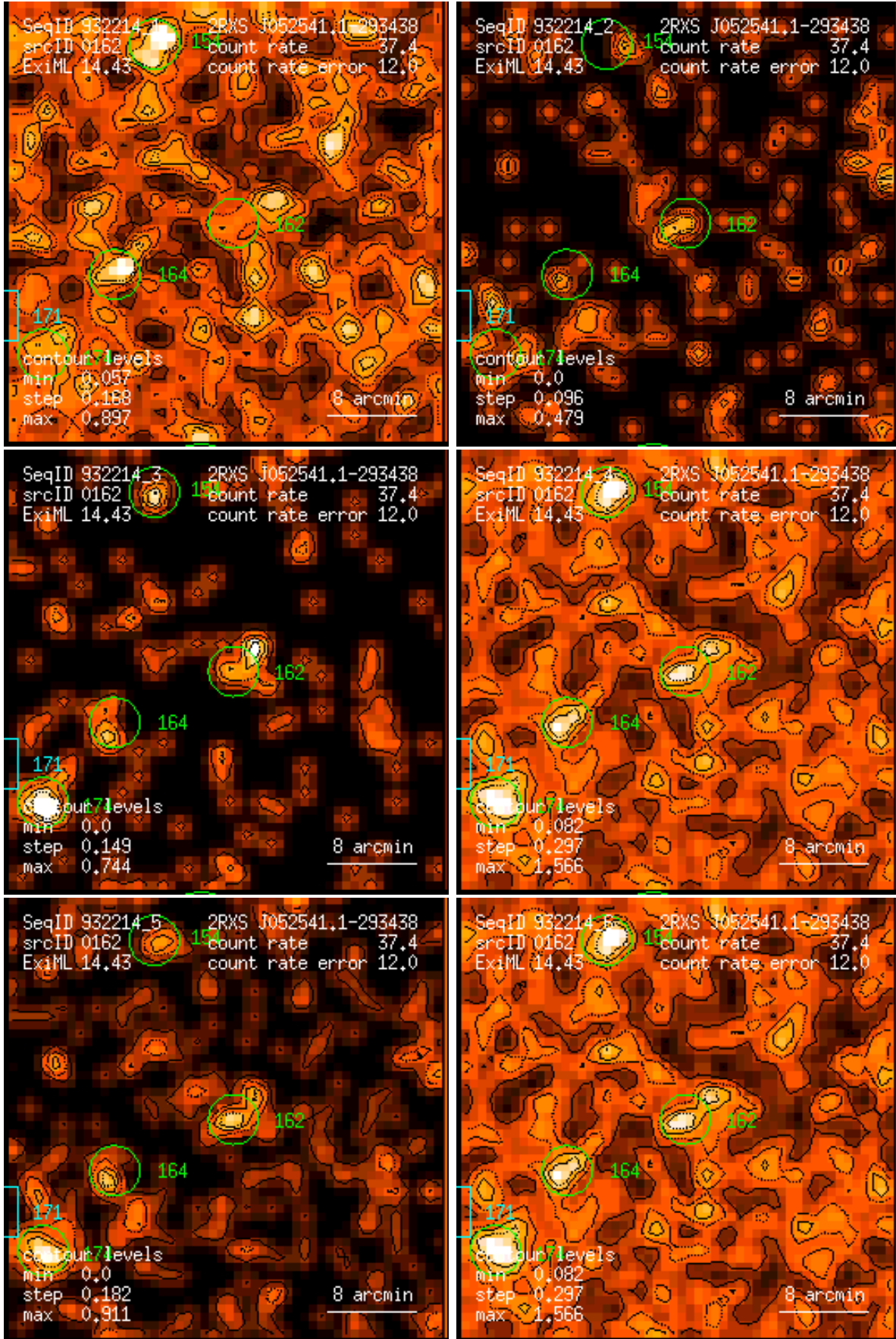
Figure 162: RASS 932214: detection 0162: band rate images, Gaussian filter: (1) PSPC channels 11 – 41, (2) 52 – 90, (3) 91 – 201, (4) 11 – 235, (5) 52 – 201, (6) 11 – 201. Broad band rates in counts/ks. Band rate contour levels in counts/ks/arcmin 2 .
