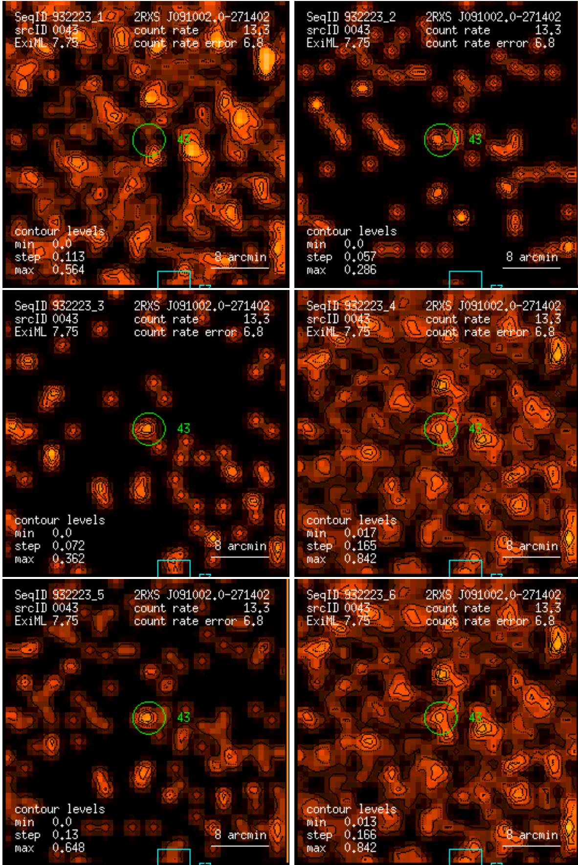
Figure 43: RASS 932223: detection 0043: band rate images, Gaussian filter: (1) PSPC channels 11 – 41, (2) 52 – 90, (3) 91 – 201, (4) 11 – 235, (5) 52 – 201, (6) 11 – 201. Broad band rates in counts/ks. Band rate contour levels in counts/ks/arcmin 2 .
