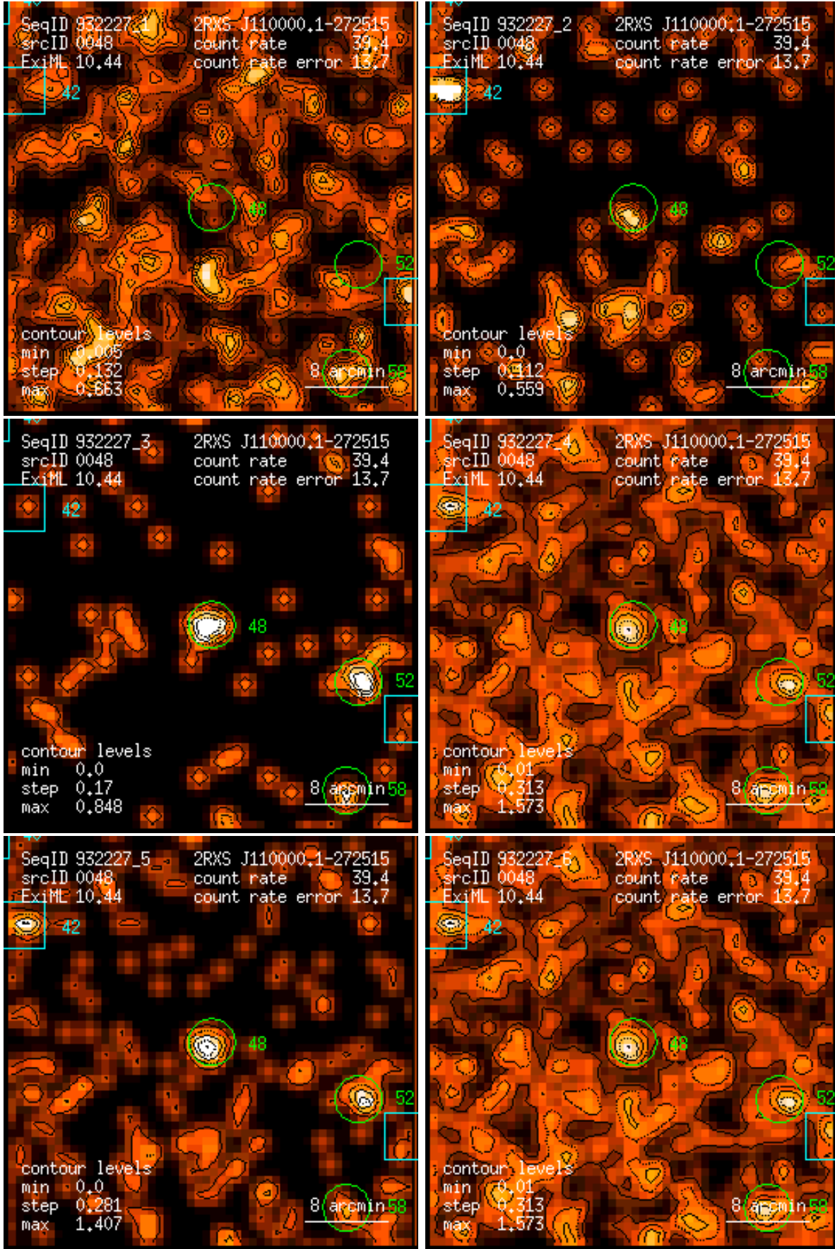
Figure 48: RASS 932227: detection 0048: band rate images, Gaussian filter: (1) PSPC channels 11 – 41, (2) 52 – 90, (3) 91 – 201, (4) 11 – 235, (5) 52 – 201, (6) 11 – 201. Broad band rates in counts/ks. Band rate contour levels in counts/ks/arcmin 2 .
