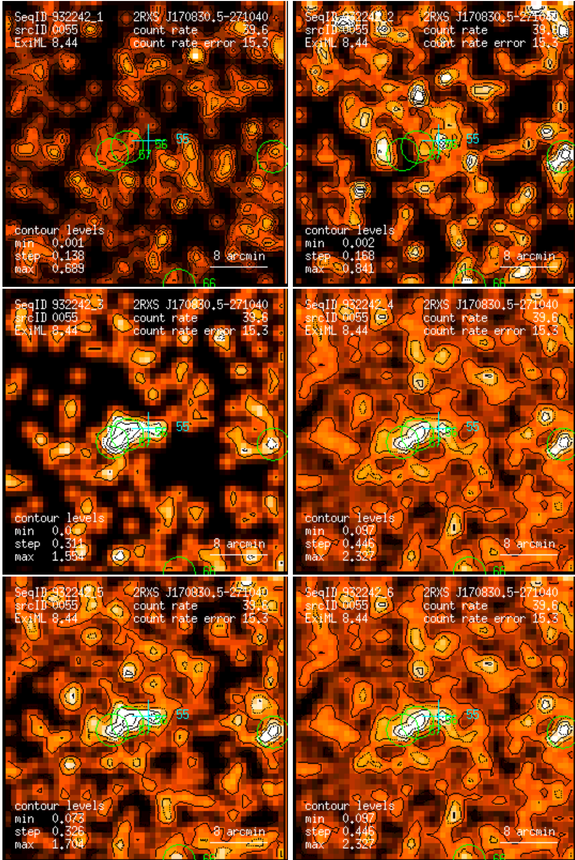
Figure 55: RASS 932242: detection 0055: band rate images, Gaussian filter: (1) PSPC channels 11 – 41, (2) 52 – 90, (3) 91 – 201, (4) 11 – 235, (5) 52 – 201, (6) 11 – 201. Broad band rates in counts/ks. Band rate contour levels in counts/ks/arcmin 2 .
