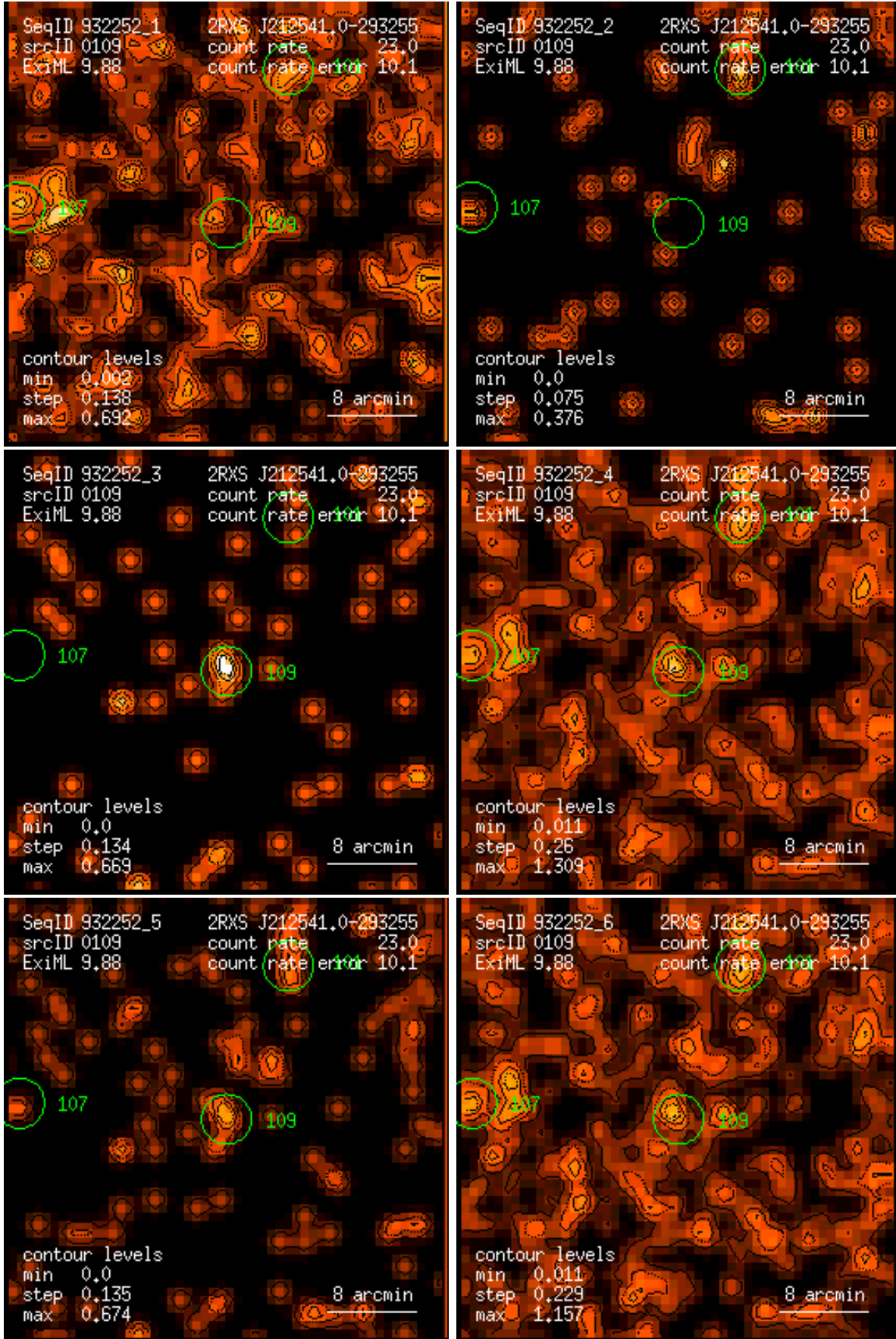
Figure 109: RASS 932252: detection 0109: band rate images, Gaussian filter: (1) PSPC channels 11 – 41, (2) 52 – 90, (3) 91 – 201, (4) 11 – 235, (5) 52 – 201, (6) 11 – 201. Broad band rates in counts/ks. Band rate contour levels in counts/ks/arcmin 2 .
