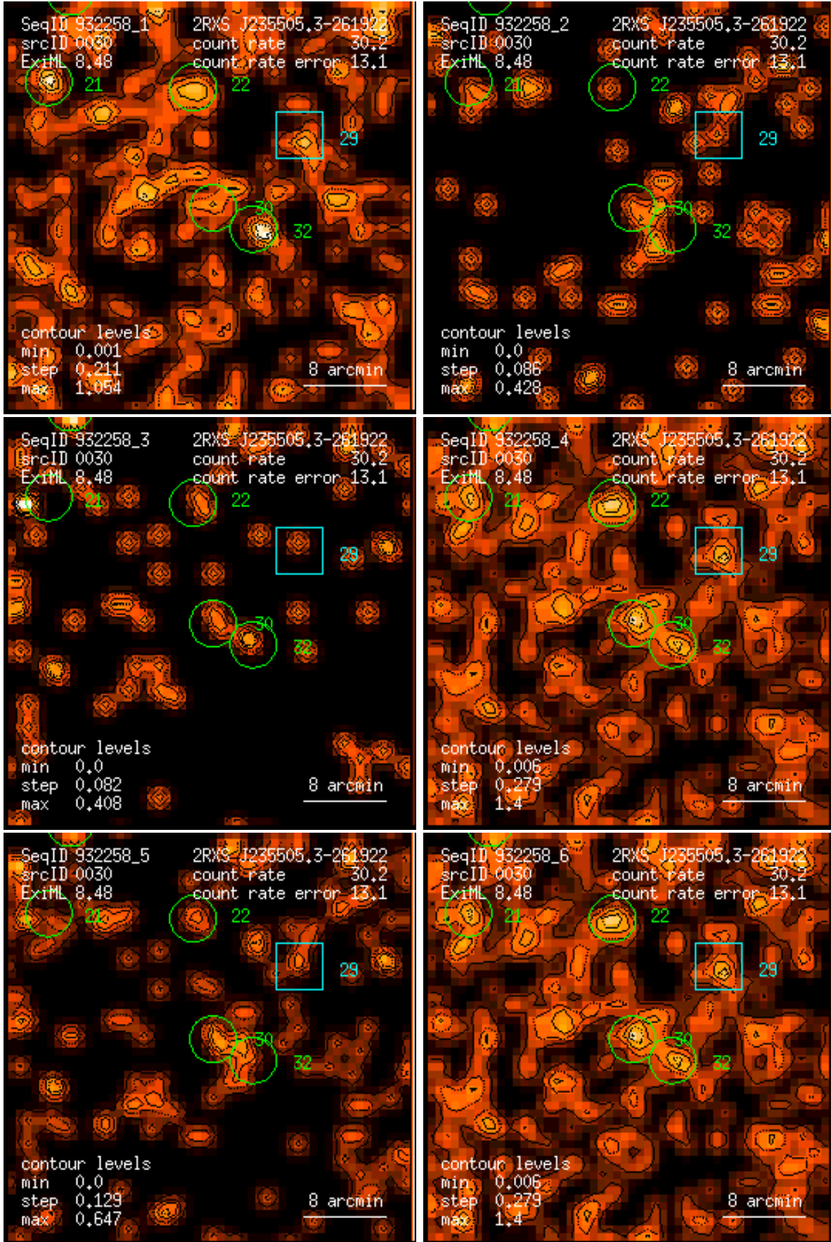
Figure 30: RASS 932258: detection 0030: band rate images, Gaussian filter: (1) PSPC channels 11 – 41, (2) 52 – 90, (3) 91 – 201, (4) 11 – 235, (5) 52 – 201, (6) 11 – 201. Broad band rates in counts/ks. Band rate contour levels in counts/ks/arcmin 2 .
