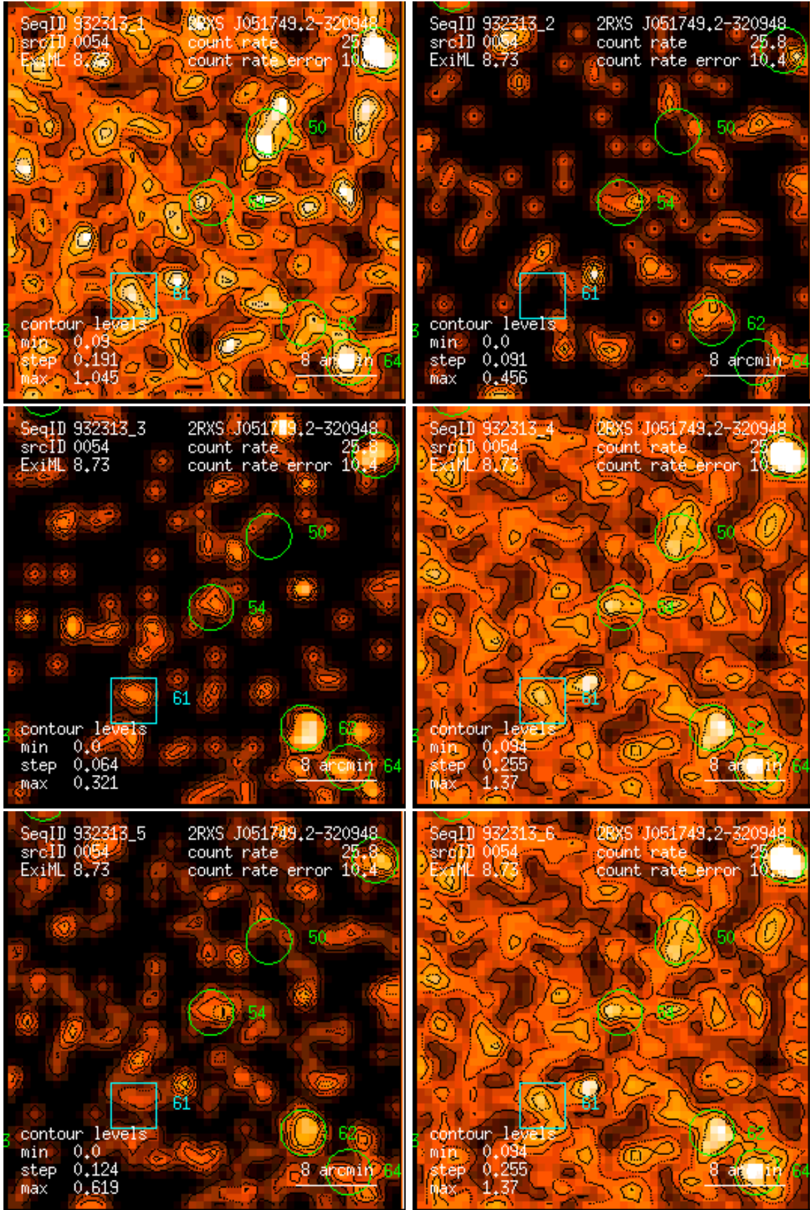
Figure 54: RASS 932313: detection 0054: band rate images, Gaussian filter: (1) PSPC channels 11 – 41, (2) 52 – 90, (3) 91 – 201, (4) 11 – 235, (5) 52 – 201, (6) 11 – 201. Broad band rates in counts/ks. Band rate contour levels in counts/ks/arcmin 2 .
