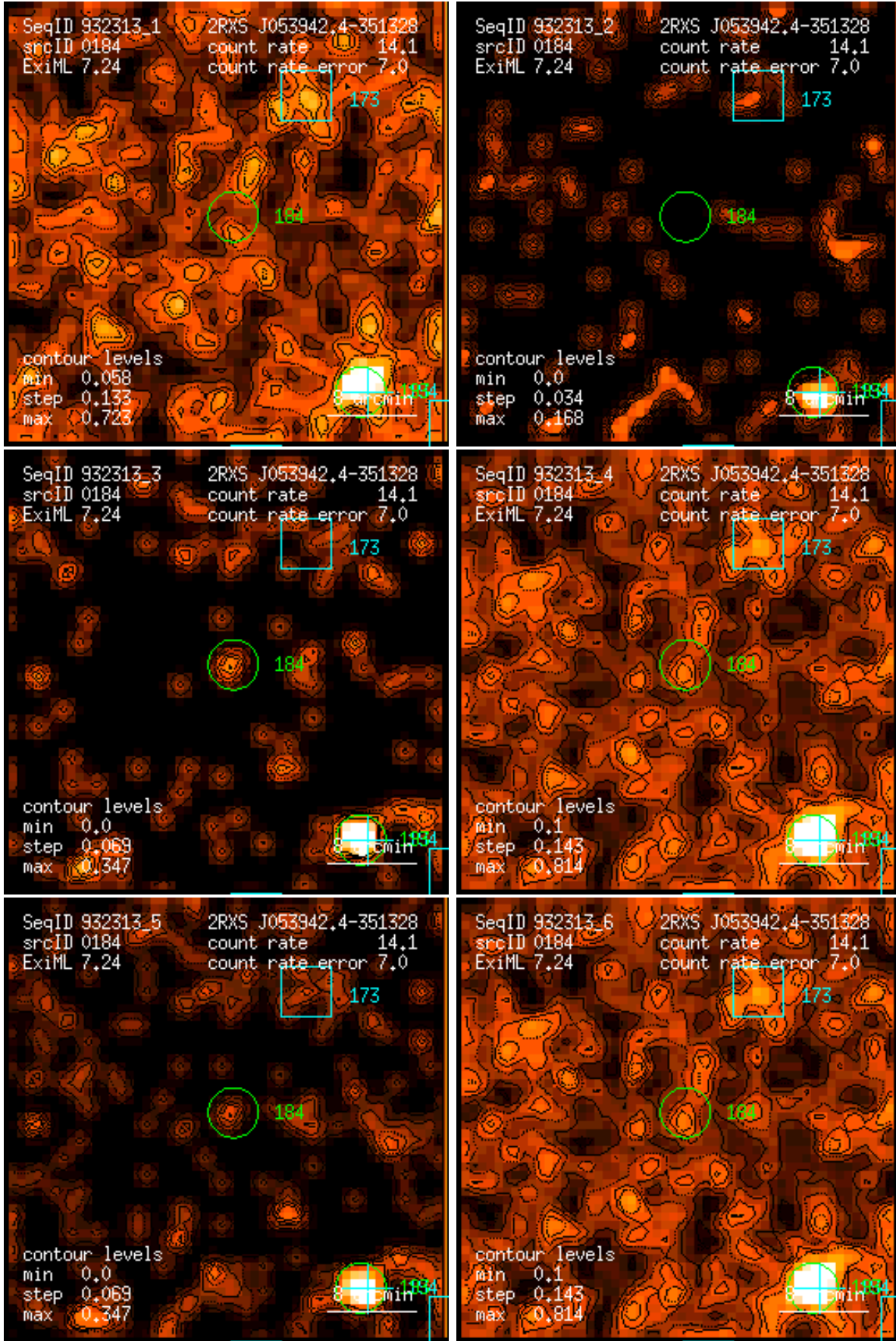
Figure 184: RASS 932313: detection 0184: band rate images, Gaussian filter: (1) PSPC channels 11 – 41, (2) 52 – 90, (3) 91 – 201, (4) 11 – 235, (5) 52 – 201, (6) 11 – 201. Broad band rates in counts/ks. Band rate contour levels in counts/ks/arcmin 2 .
