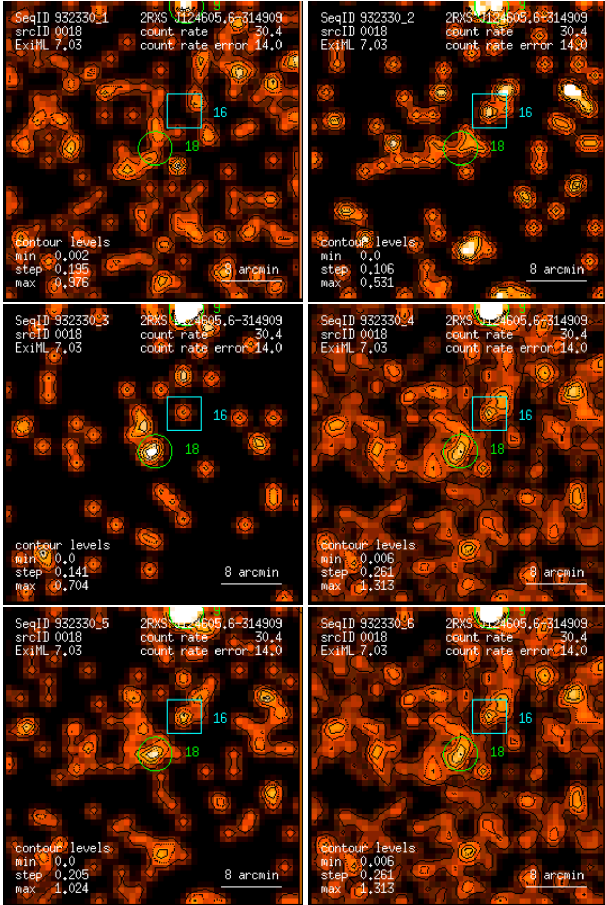
Figure 18: RASS 932330: detection 0018: band rate images, Gaussian filter: (1) PSPC channels 11 – 41, (2) 52 – 90, (3) 91 – 201, (4) 11 – 235, (5) 52 – 201, (6) 11 – 201. Broad band rates in counts/ks. Band rate contour levels in counts/ks/arcmin 2 .
