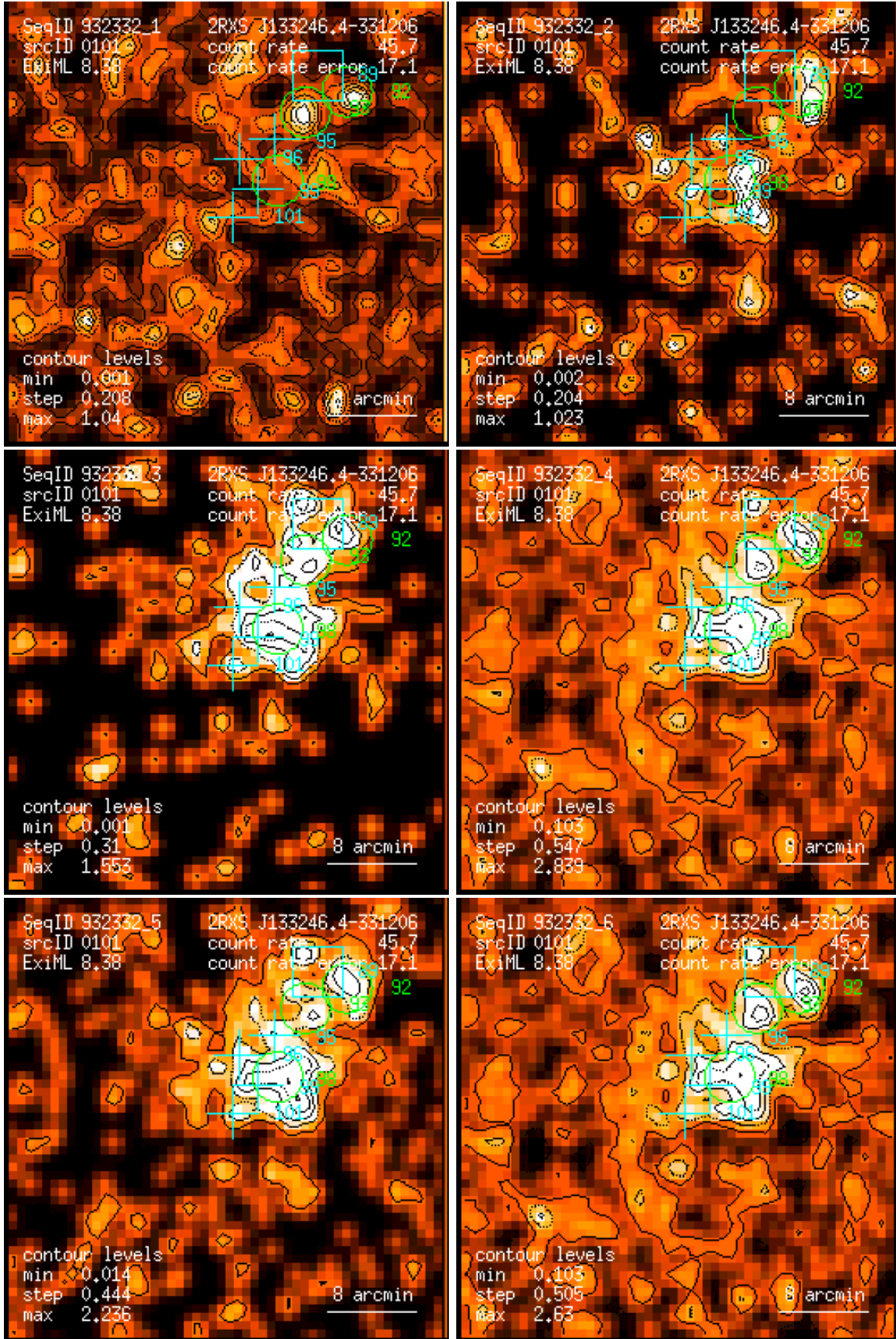
Figure 101: RASS 932332: detection 0101: band rate images, Gaussian filter: (1) PSPC channels 11 – 41, (2) 52 – 90, (3) 91 – 201, (4) 11 – 235, (5) 52 – 201, (6) 11 – 201. Broad band rates in counts/ks. Band rate contour levels in counts/ks/arcmin 2 .
