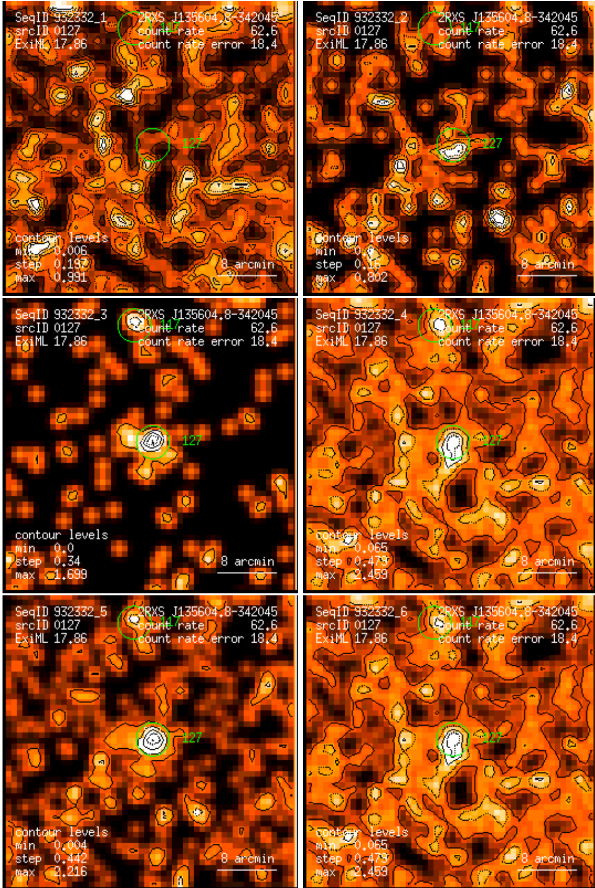
Figure 127: RASS 932332: detection 0127: band rate images, Gaussian filter: (1) PSPC channels 11 – 41, (2) 52 – 90, (3) 91 – 201, (4) 11 – 235, (5) 52 – 201, (6) 11 – 201. Broad band rates in counts/ks. Band rate contour levels in counts/ks/arcmin 2 .
