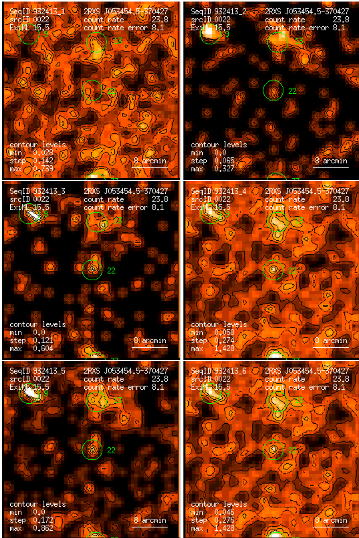
Figure 22: RASS 932413: detection 0022: band rate images, Gaussian filter: (1) PSPC channels 11 – 41, (2) 52 – 90, (3) 91 – 201, (4) 11 – 235, (5) 52 – 201, (6) 11 – 201. Broad band rates in counts/ks. Band rate contour levels in counts/ks/arcmin 2 .
