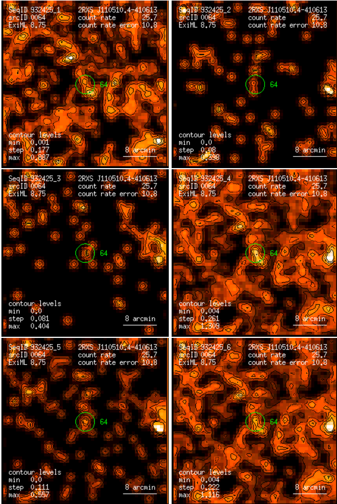
Figure 64: RASS 932425: detection 0064: band rate images, Gaussian filter: (1) PSPC channels 11 – 41, (2) 52 – 90, (3) 91 – 201, (4) 11 – 235, (5) 52 – 201, (6) 11 – 201. Broad band rates in counts/ks. Band rate contour levels in counts/ks/arcmin 2 .
