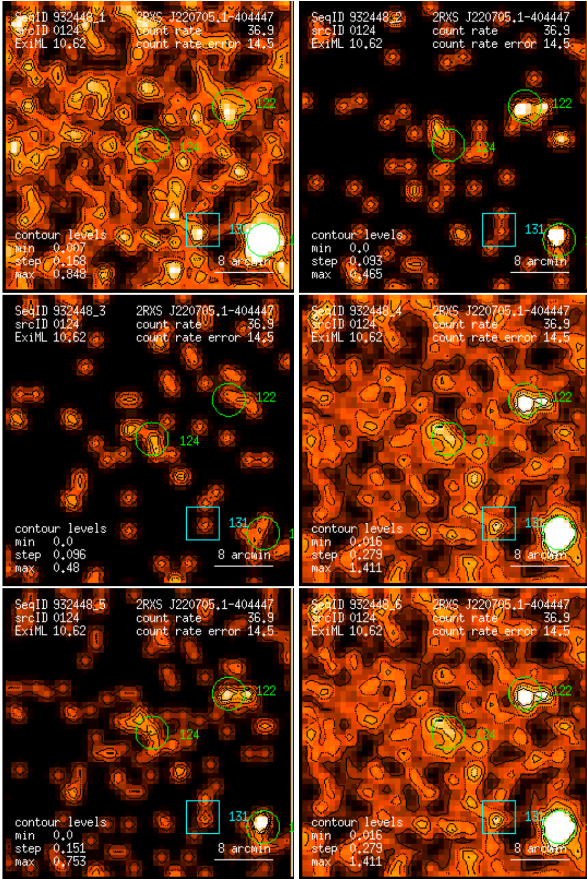
Figure 124: RASS 932448: detection 0124: band rate images, Gaussian filter: (1) PSPC channels 11 – 41, (2) 52 – 90, (3) 91 – 201, (4) 11 – 235, (5) 52 – 201, (6) 11 – 201. Broad band rates in counts/ks. Band rate contour levels in counts/ks/arcmin 2 .
