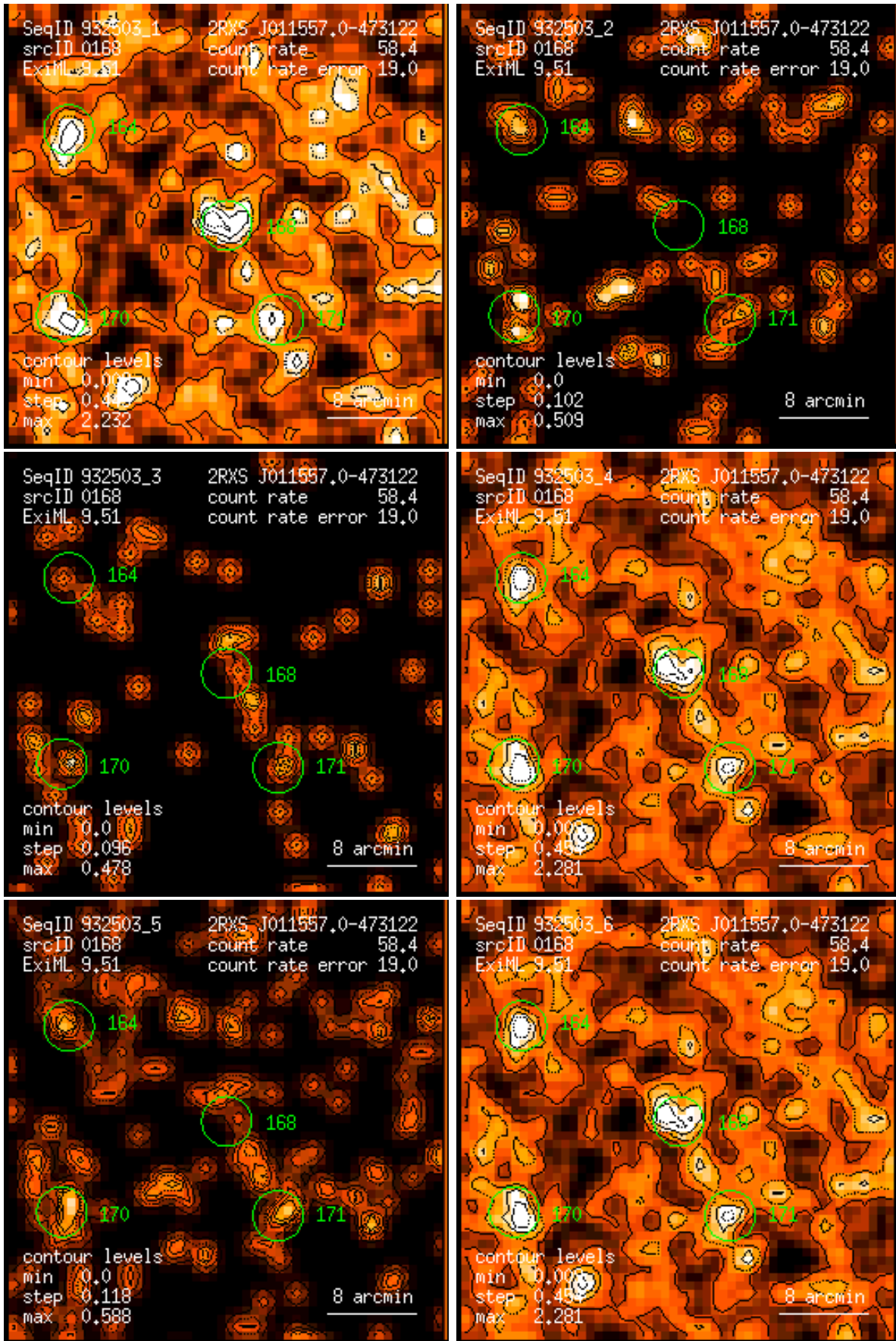
Figure 168: RASS 932503: detection 0168: band rate images, Gaussian filter: (1) PSPC channels 11 – 41, (2) 52 – 90, (3) 91 – 201, (4) 11 – 235, (5) 52 – 201, (6) 11 – 201. Broad band rates in counts/ks. Band rate contour levels in counts/ks/arcmin 2 .
