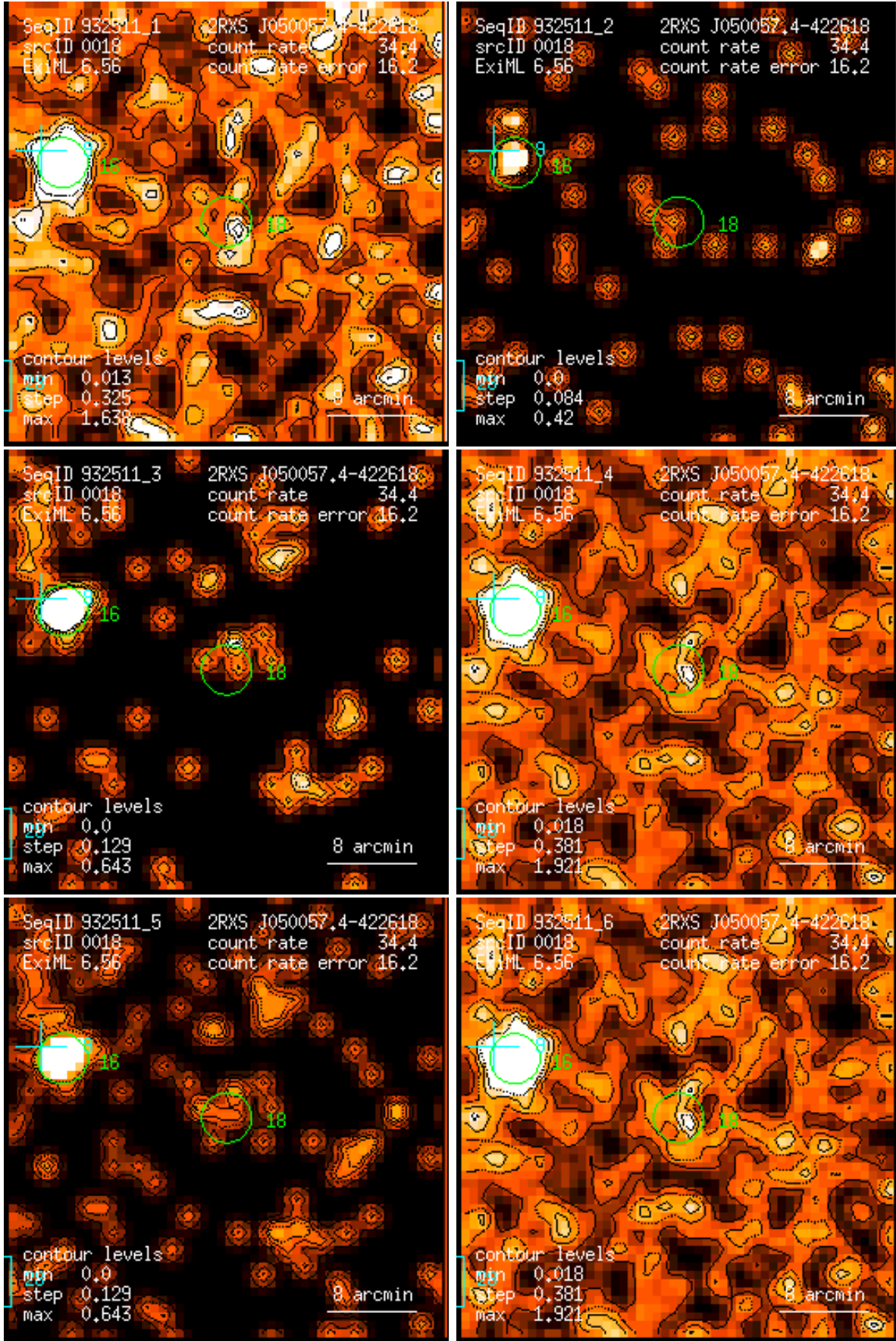
Figure 18: RASS 932511: detection 0018: band rate images, Gaussian filter: (1) PSPC channels 11 – 41, (2) 52 – 90, (3) 91 – 201, (4) 11 – 235, (5) 52 – 201, (6) 11 – 201. Broad band rates in counts/ks. Band rate contour levels in counts/ks/arcmin 2 .
