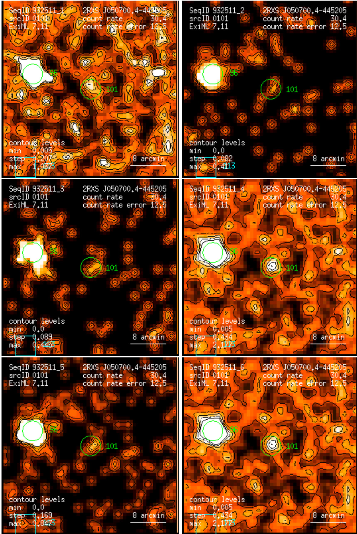
Figure 101: RASS 932511: detection 0101: band rate images, Gaussian filter: (1) PSPC channels 11 – 41, (2) 52 – 90, (3) 91 – 201, (4) 11 – 235, (5) 52 – 201, (6) 11 – 201. Broad band rates in counts/ks. Band rate contour levels in counts/ks/arcmin 2 .
