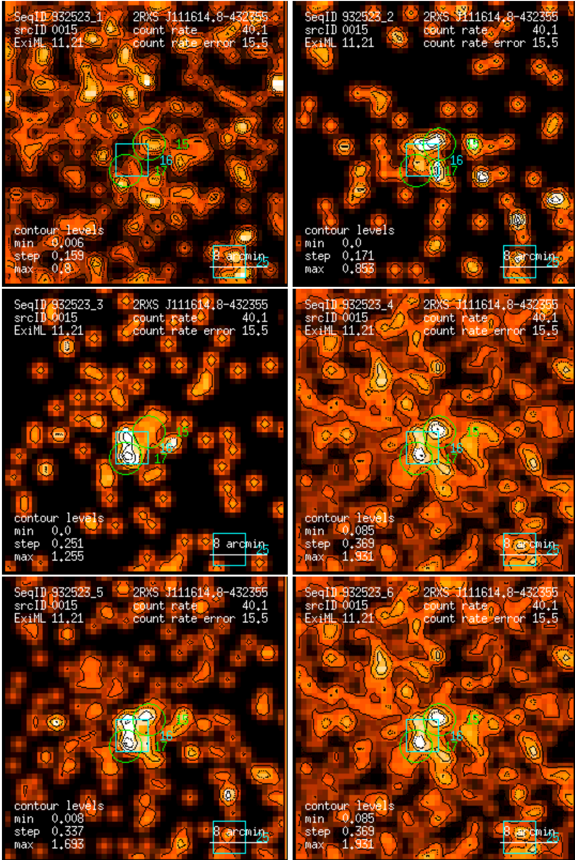
Figure 15: RASS 932523: detection 0015: band rate images, Gaussian filter: (1) PSPC channels 11 – 41, (2) 52 – 90, (3) 91 – 201, (4) 11 – 235, (5) 52 – 201, (6) 11 – 201. Broad band rates in counts/ks. Band rate contour levels in counts/ks/arcmin 2 .
