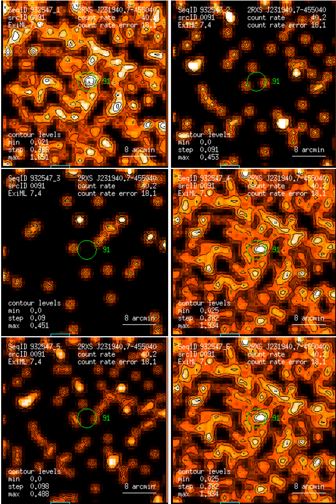
Figure 91: RASS 932547: detection 0091: band rate images, Gaussian filter: (1) PSPC channels 11 – 41, (2) 52 – 90, (3) 91 – 201, (4) 11 – 235, (5) 52 – 201, (6) 11 – 201. Broad band rates in counts/ks. Band rate contour levels in counts/ks/arcmin 2 .
