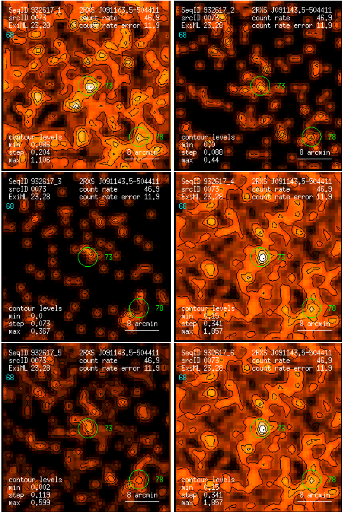
Figure 73: RASS 932617: detection 0073: band rate images, Gaussian filter: (1) PSPC channels 11 – 41, (2) 52 – 90, (3) 91 – 201, (4) 11 – 235, (5) 52 – 201, (6) 11 – 201. Broad band rates in counts/ks. Band rate contour levels in counts/ks/arcmin 2 .
