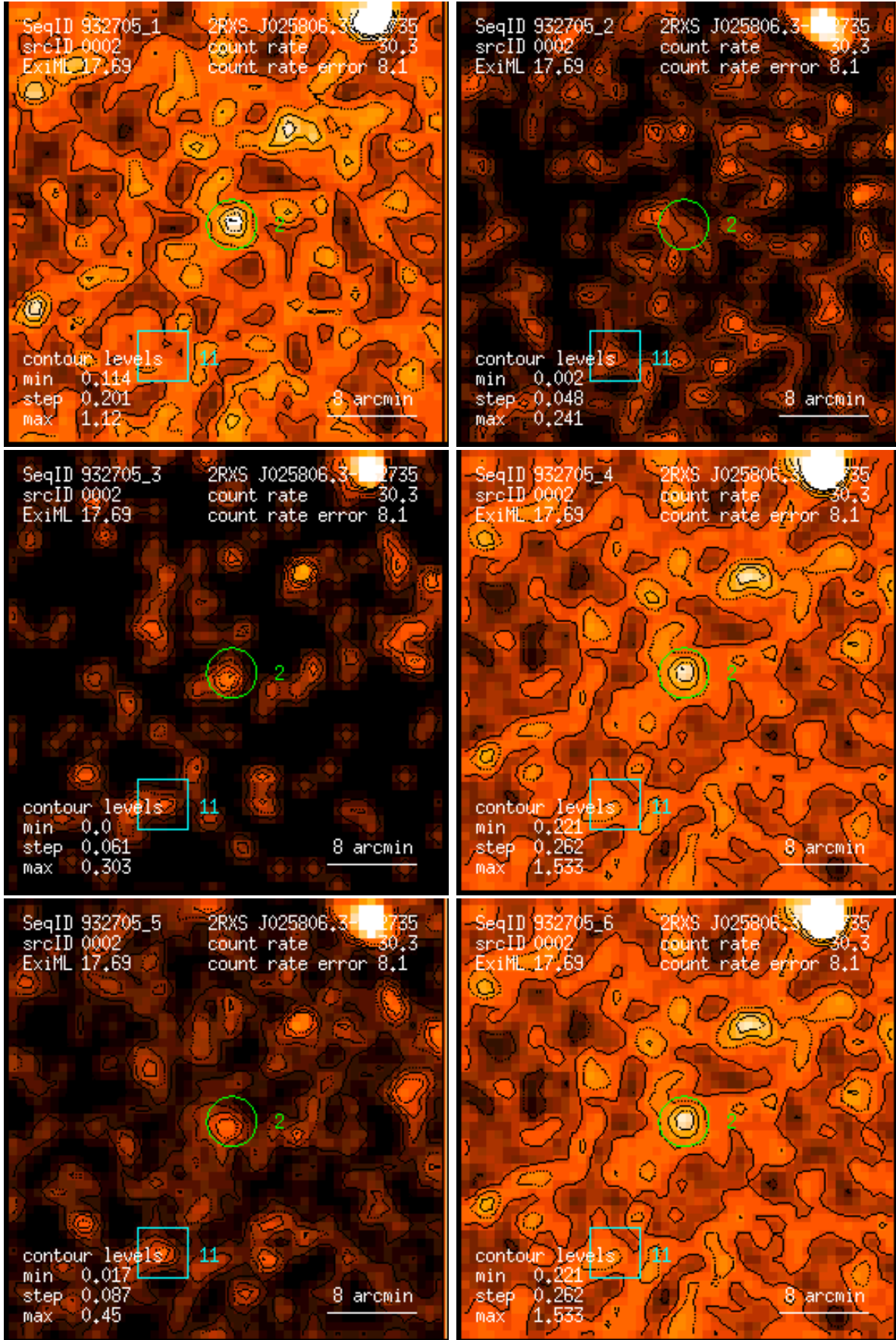
Figure 2: RASS 932705: detection 0002: band rate images, Gaussian filter: (1) PSPC channels 11 – 41, (2) 52 – 90, (3) 91 – 201, (4) 11 – 235, (5) 52 – 201, (6) 11 – 201. Broad band rates in counts/ks. Band rate contour levels in counts/ks/arcmin 2 .
