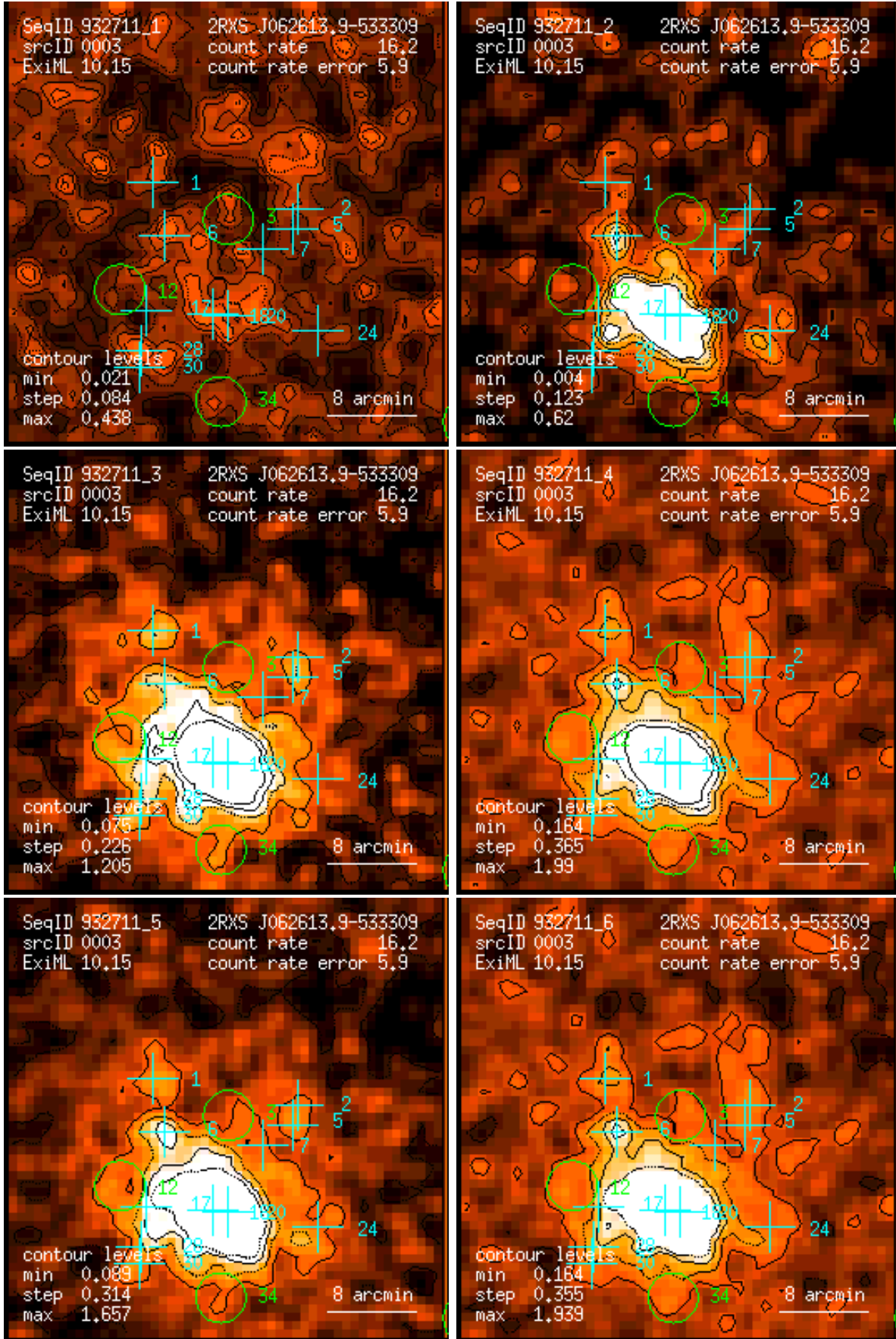
Figure 3: RASS 932711: detection 0003: band rate images, Gaussian filter: (1) PSPC channels 11 – 41, (2) 52 – 90, (3) 91 – 201, (4) 11 – 235, (5) 52 – 201, (6) 11 – 201. Broad band rates in counts/ks. Band rate contour levels in counts/ks/arcmin 2 .
