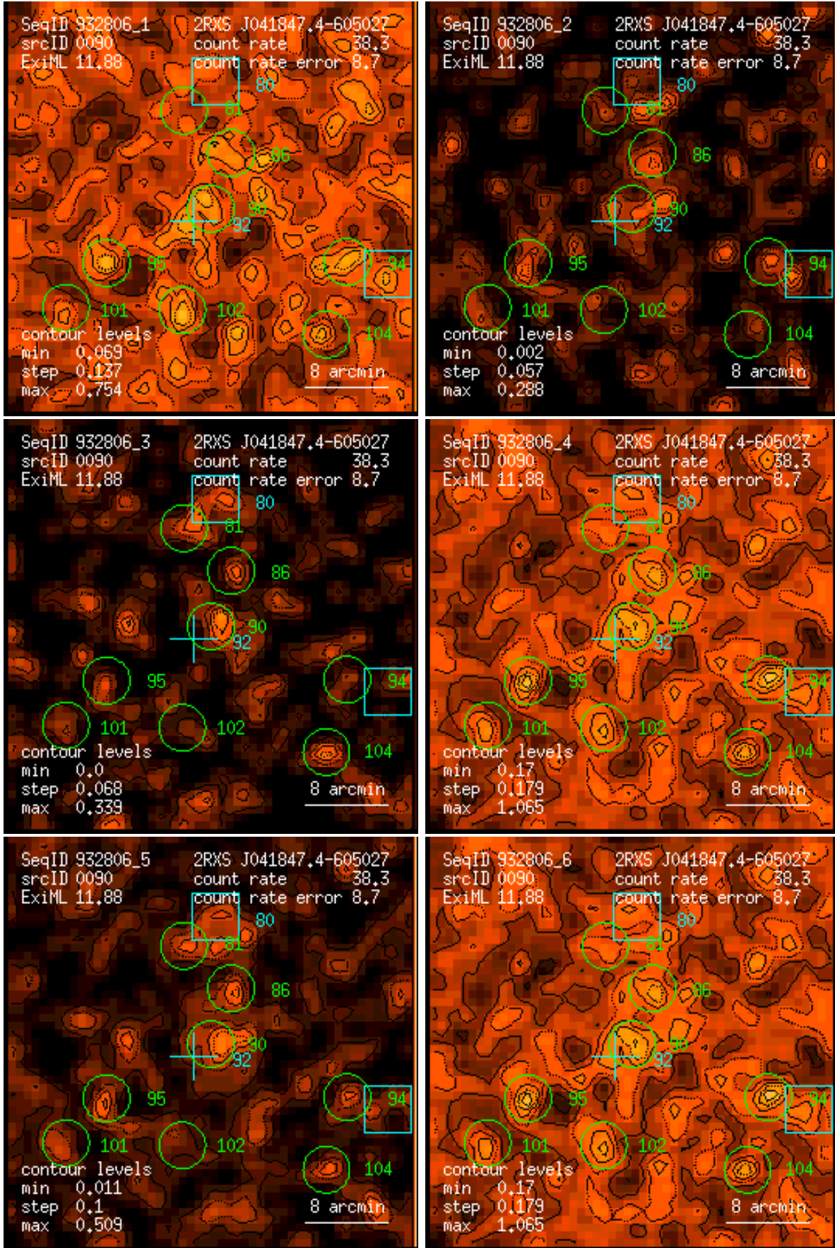
Figure 90: RASS 932806: detection 0090: band rate images, Gaussian filter: (1) PSPC channels 11 – 41, (2) 52 – 90, (3) 91 – 201, (4) 11 – 235, (5) 52 – 201, (6) 11 – 201. Broad band rates in counts/ks. Band rate contour levels in counts/ks/arcmin 2 .
