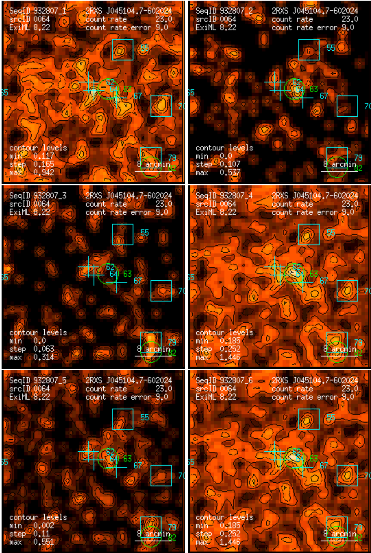
Figure 64: RASS 932807: detection 0064: band rate images, Gaussian filter: (1) PSPC channels 11 – 41, (2) 52 – 90, (3) 91 – 201, (4) 11 – 235, (5) 52 – 201, (6) 11 – 201. Broad band rates in counts/ks. Band rate contour levels in counts/ks/arcmin 2 .
